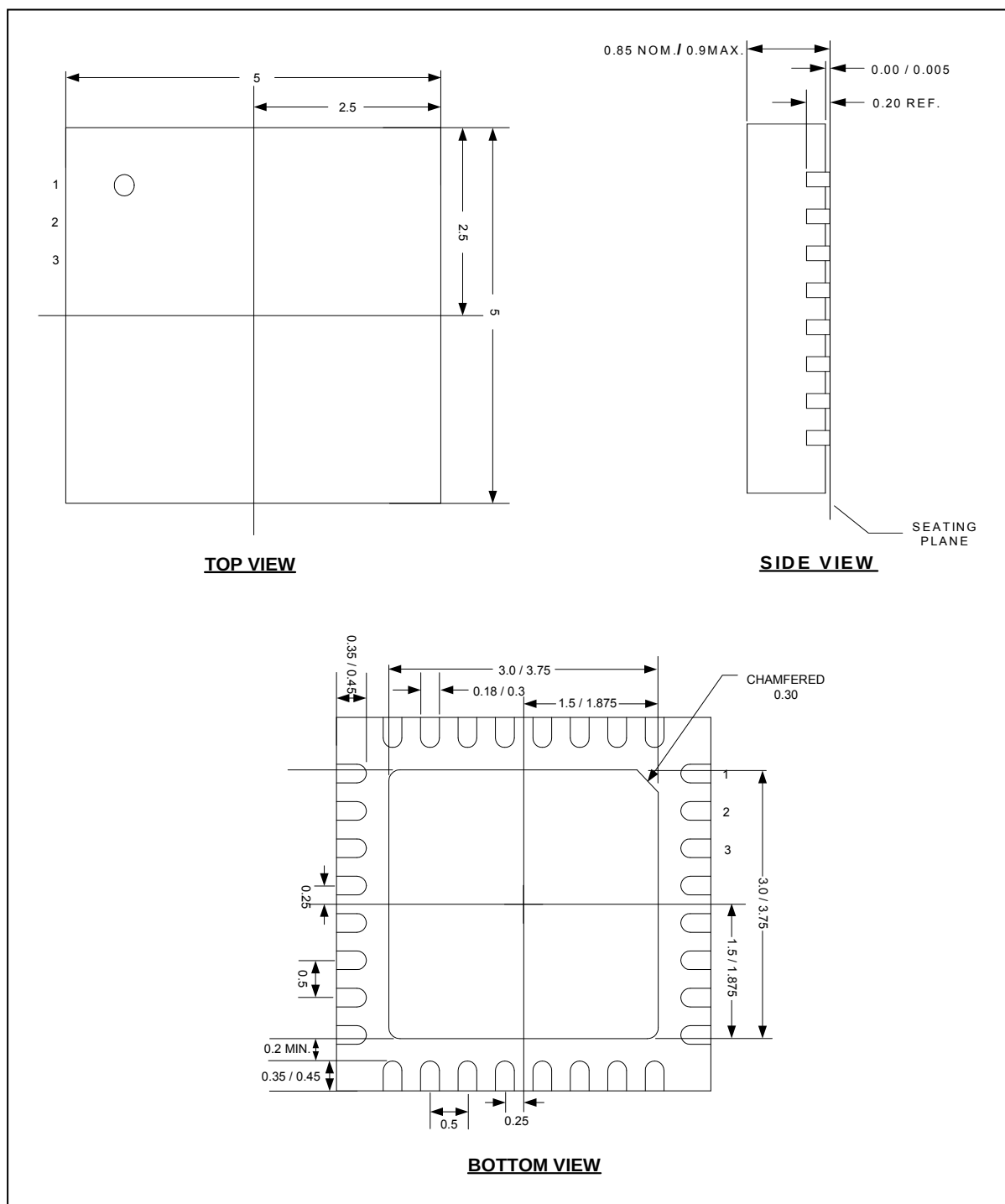
Figure 14: 32-pin QFN Package Drawing
