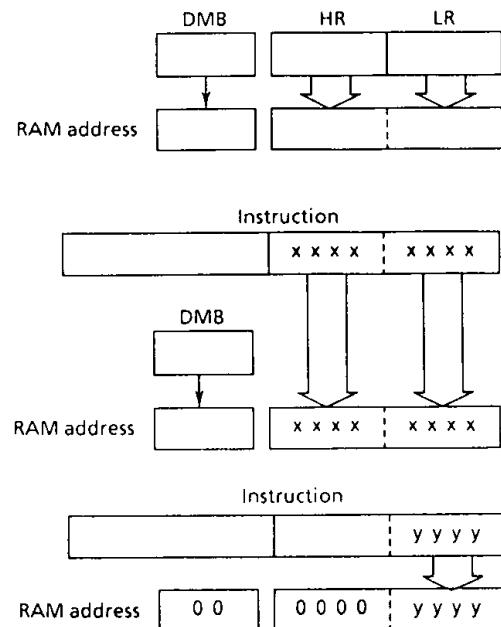
Figure 2-5. Addressing mode
