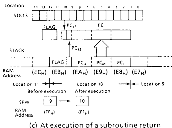
Figure 2-7. Accessing Stack (Save/Restore)
