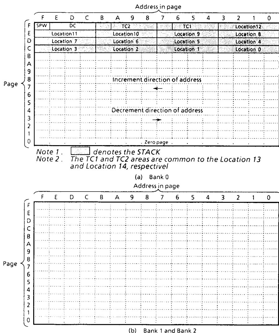
Figure 2-6. Data Memory Map
