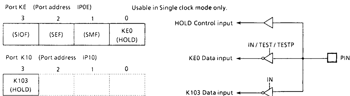
Figure 3-12. Port KE
