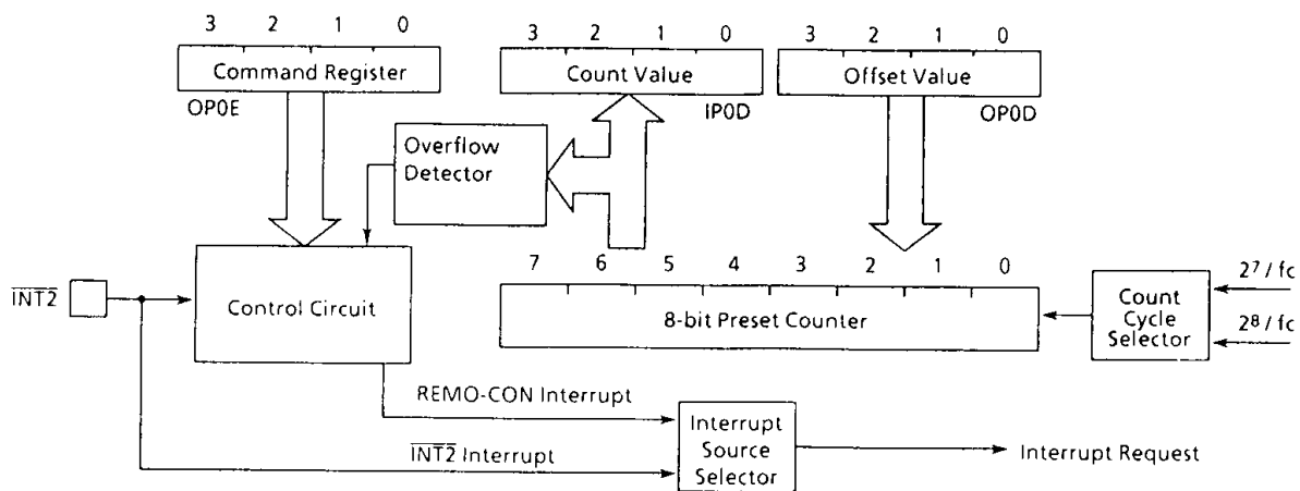
Figure 3-26. Remote Control Pre-processor
