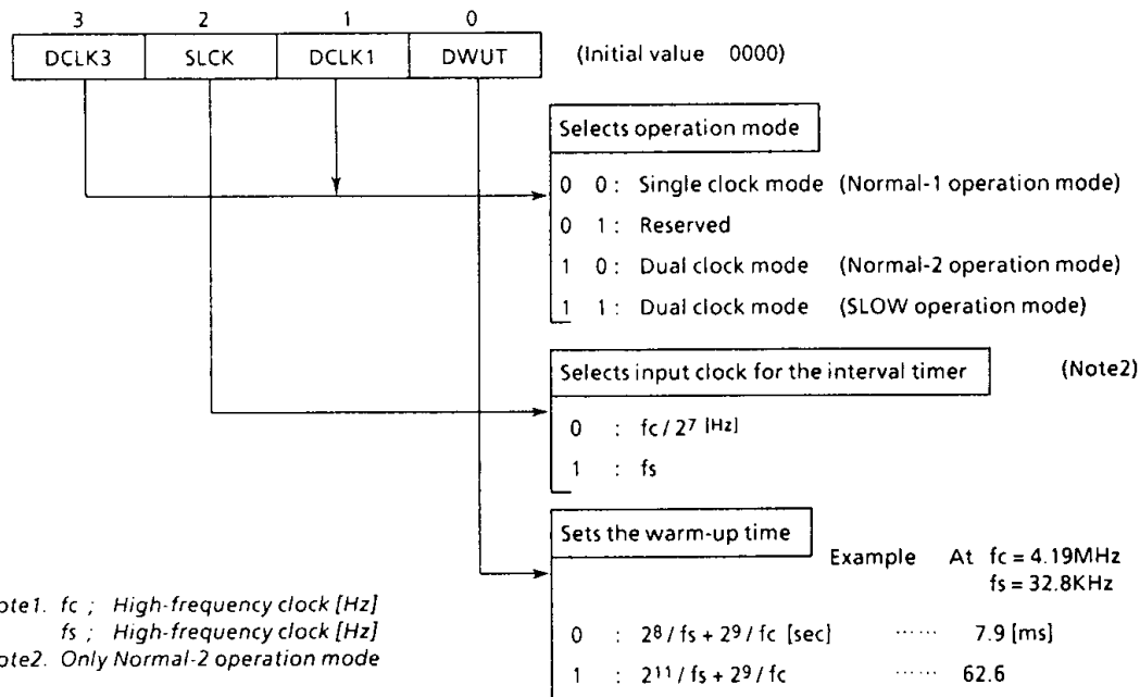
Figure 2-17. System Clock Control Command Register
