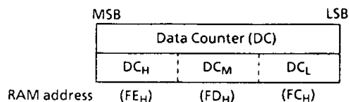
Figure 2-9. Data Counter
