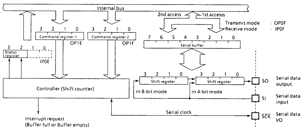
Figure 3-29. Configuration of Serial Interface
