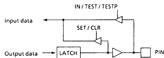
Figure 3-11. Ports RA, RB, RC
