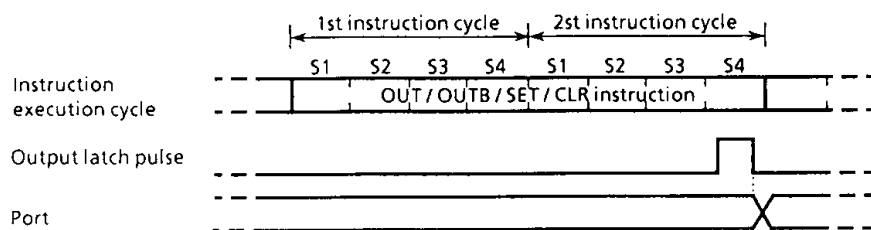
Figure 3-2. Output Timing
