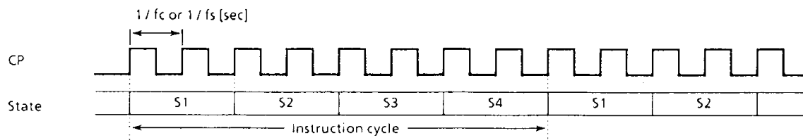
Figure 2-20. Instruction Cycle
