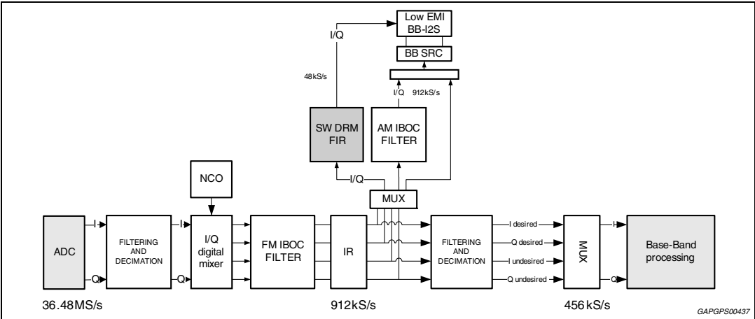
Figure 13. Digital-down-converter simplified block diagram
