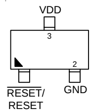
SOT-23-3 (L-Type)
