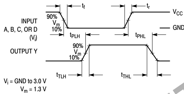
Figure 2. Switching Waveforms
