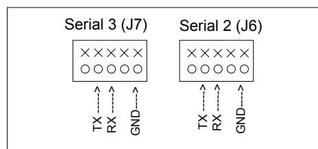
Figure 2. DS5250 Revision A Showing Pinout of J6 and J7
