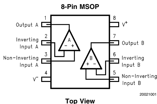
Connection Diagram
