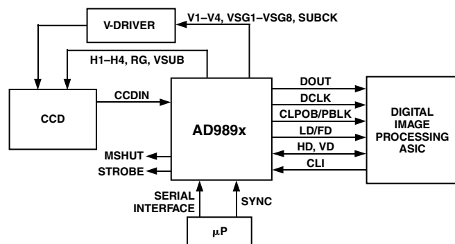
Figure 5. Typical System Block Diagram, Master Mode
