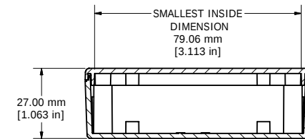
SECTION R-R
