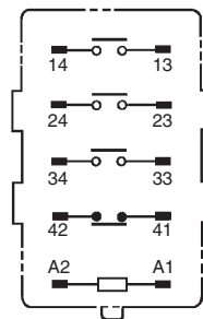
G7J-3A1B-P(B)(T)
