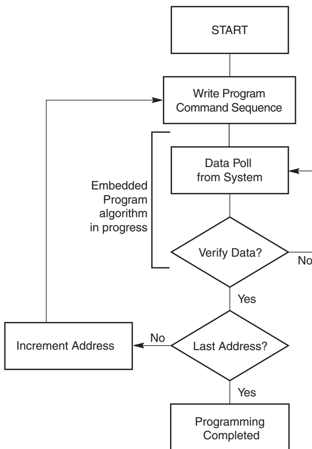
Figure 11.1 Program Operation
