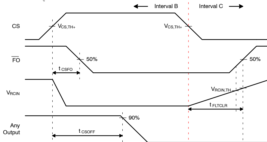
Figure 36. Detailed View of B and C Intervals During Over-Current Protection
