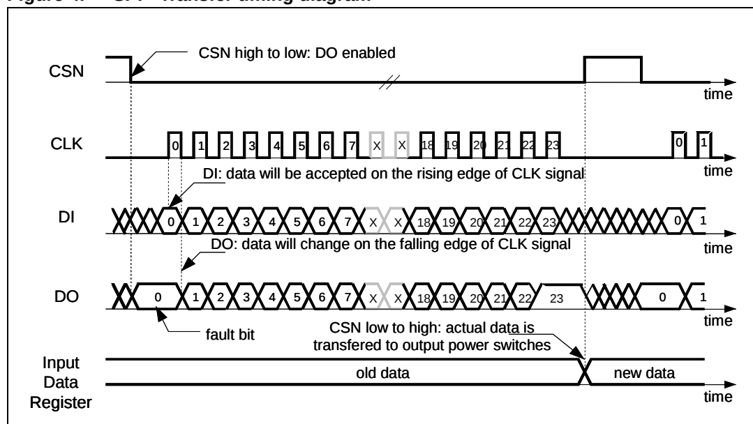
Figure 4. SPI - Transfer timing diagram
