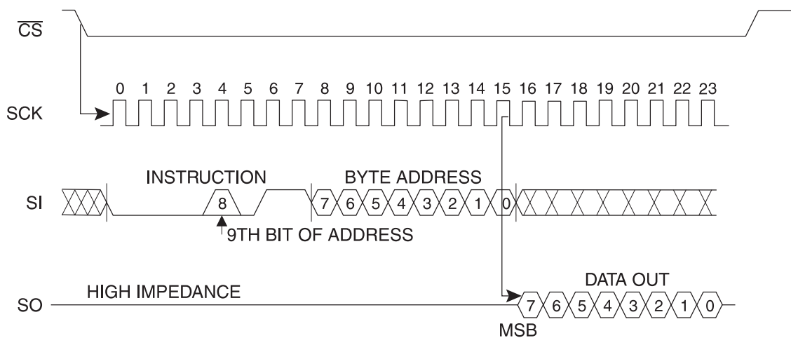
Figure 8. READ Timing
