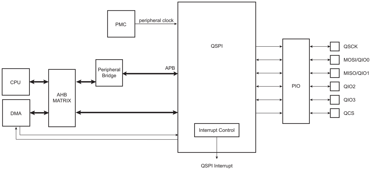
Figure 50-1: Block Diagram
