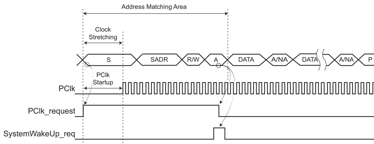
Figure 46-44: Address Match Only (Data Matching Disabled)
