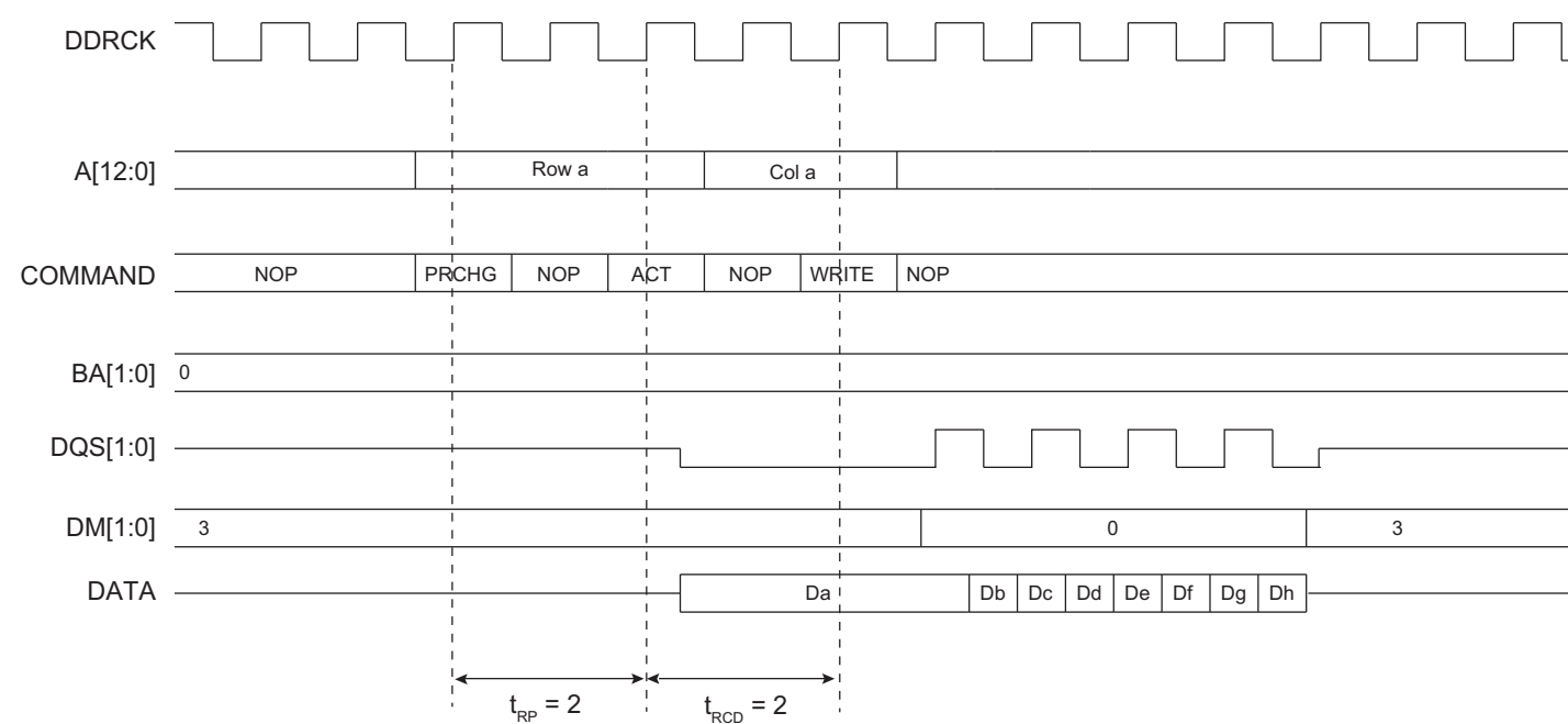
Figure 36-4: Burst Write Access, Row Closed, DDR-SDRAM Devices
