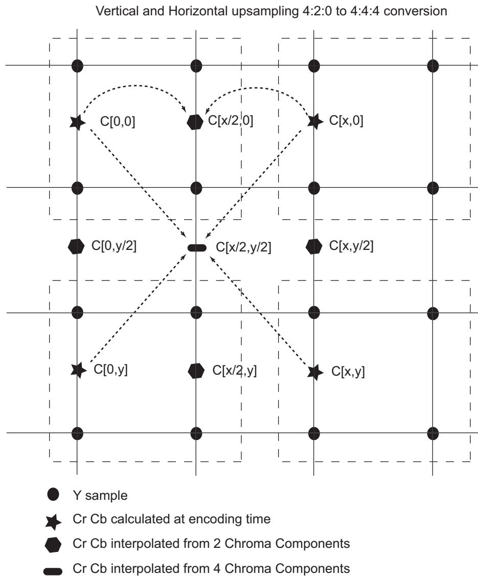
Figure 39-5: 4:2:0 Upsampling Algorithm
