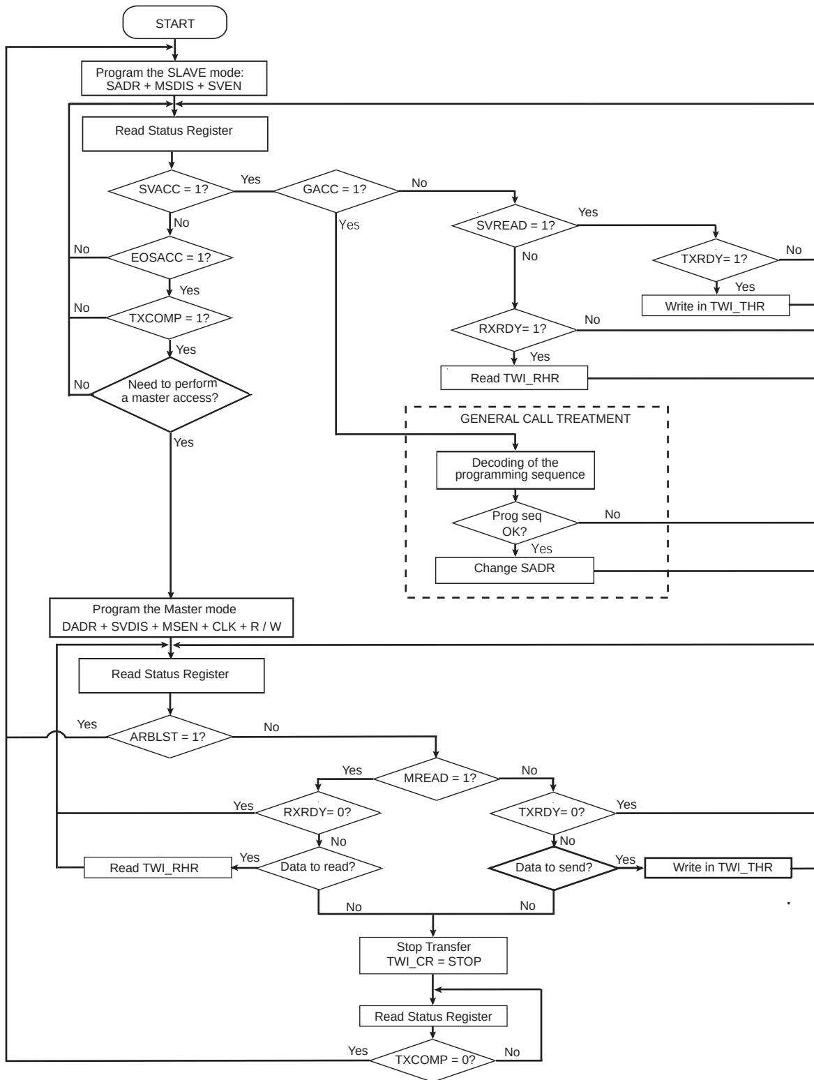
Figure 46-35: Multimaster Flowchart
