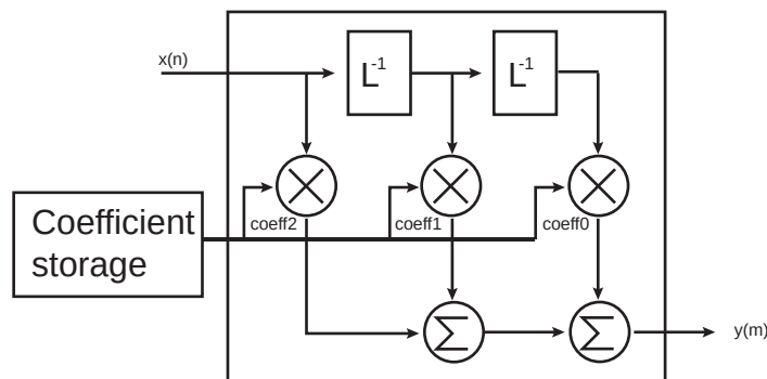
Figure 39-8: Vertical Resampler Filter Architecture
