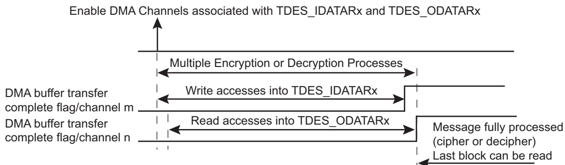
Figure 62-3: DMA Transfer with LOD = 0
