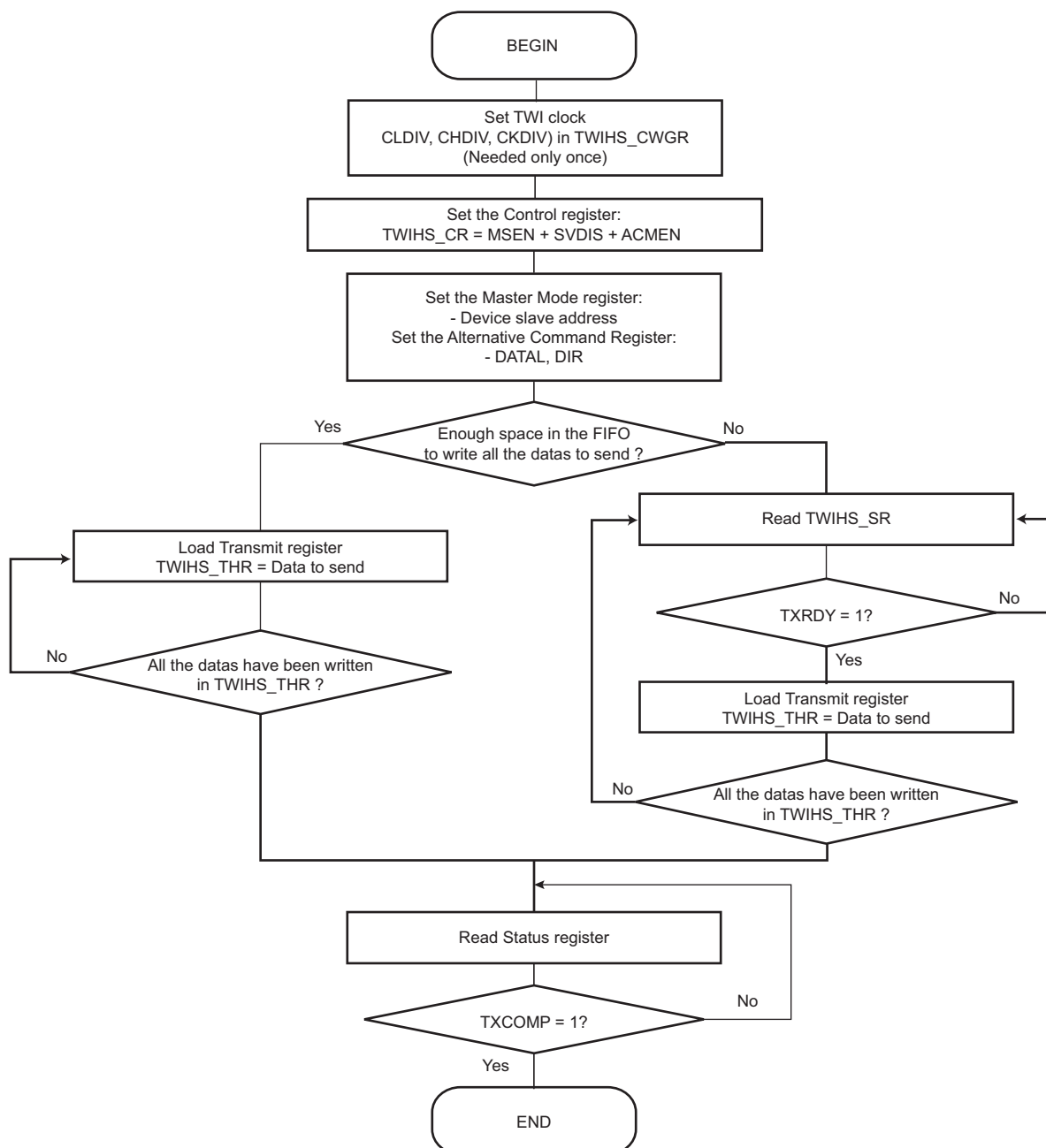
Figure 46-29: Sending Data with FIFO Flowchart
