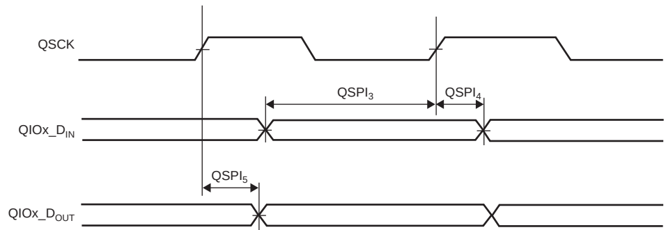
Figure 66-27: QSPI Master Mode 1
