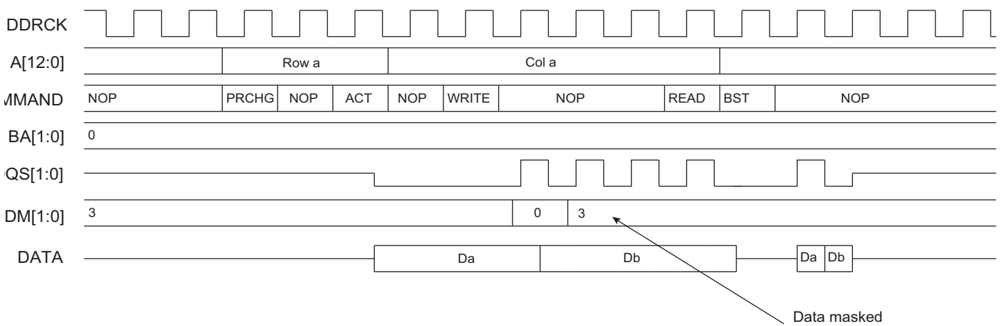
Figure 36-7: SINGLE Write Access Followed by a Read Access, DDR-SDRAM Devices
