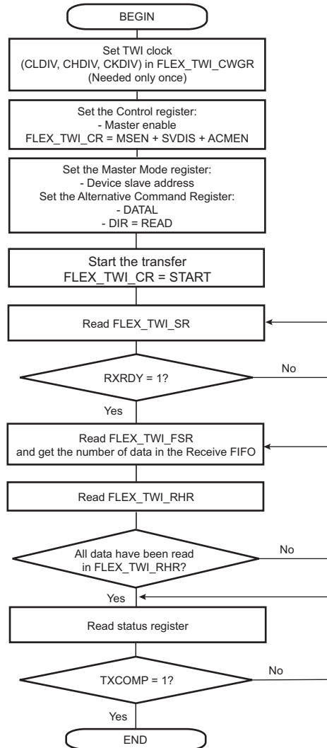
Figure 47-130: Receiving Data with FIFO Enabled in Master Mode
