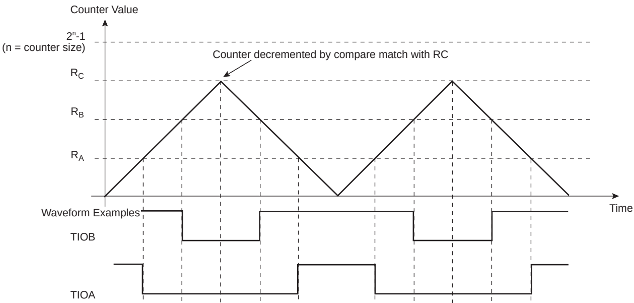
Figure 54-14: WAVSEL = 11 without Trigger
