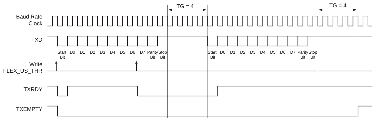
Figure 47-22: Timeguard Operations
