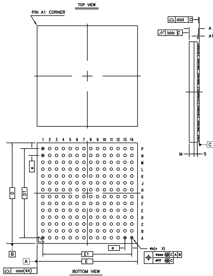
Figure 67-3: 196-ball TFBGA Package Details
