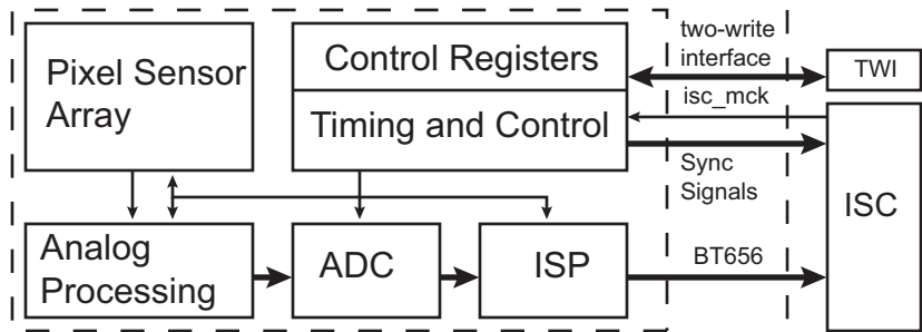
Figure 52-6: BT656 Video Interface Sensor
