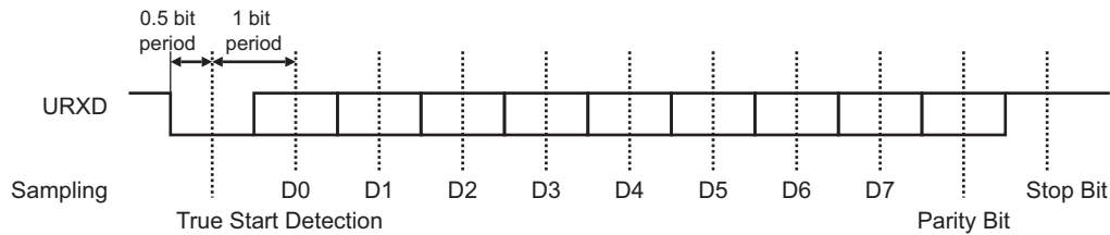
Figure 48-4: Character Reception
