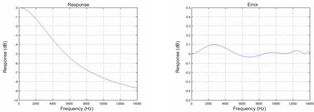
Figure 43-8: De-emphasis Filter: Frequency Response & Error ( f_s = 32 kHz)
