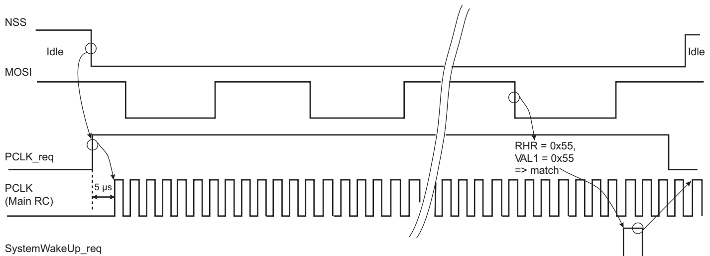
Figure 49-14: Asynchronous Wakeup Use Case Example
