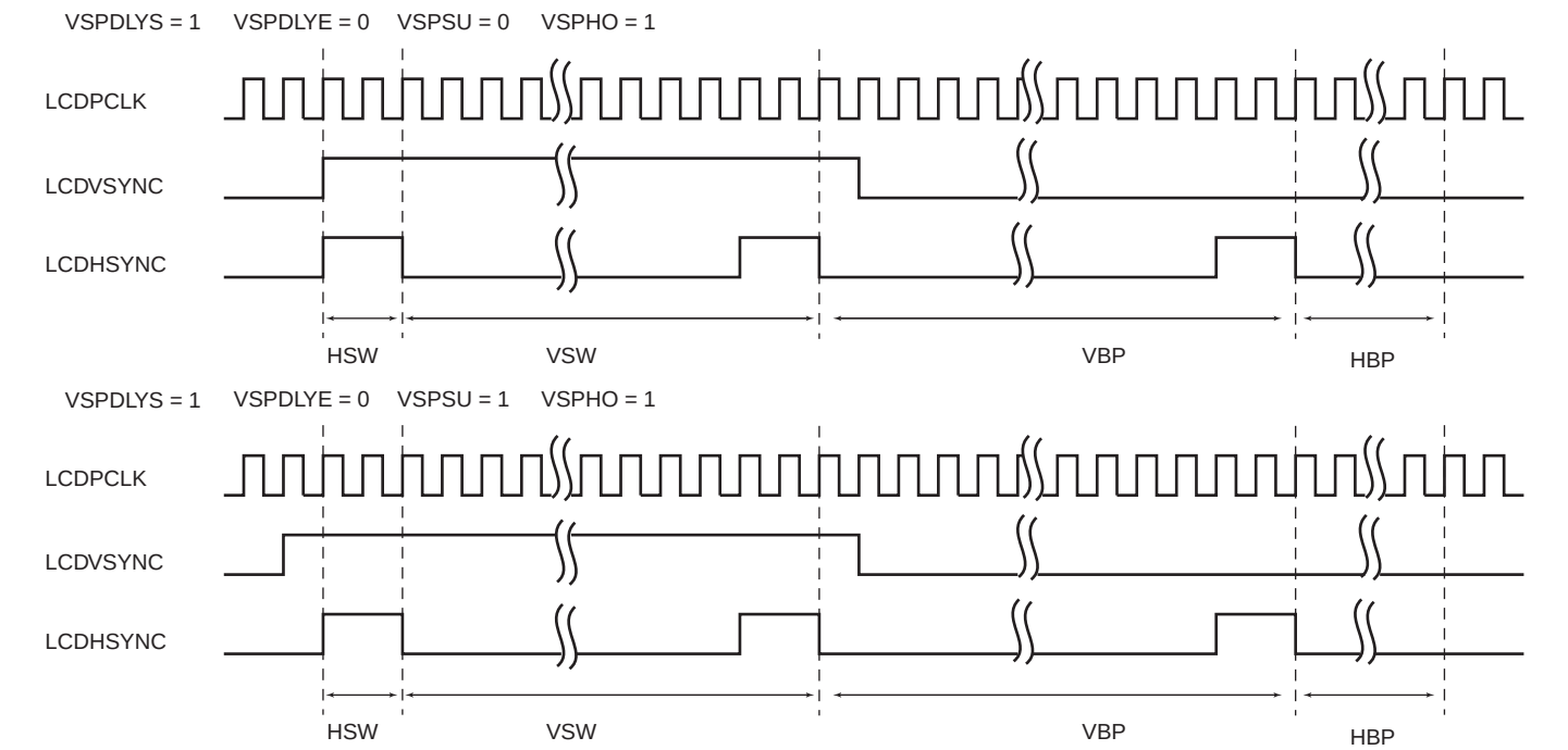
Figure 39-16: Vertical Synchronization Timing (part 2)
