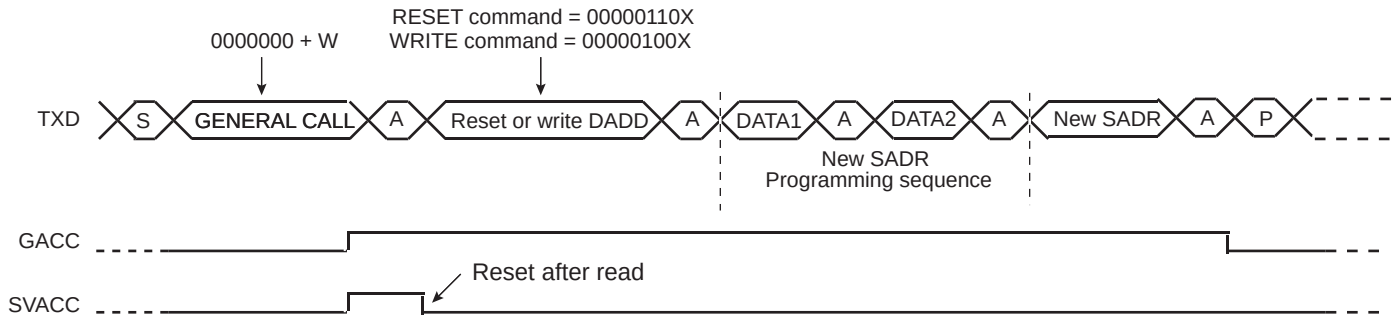
Figure 46-38: Master Performs a General Call
