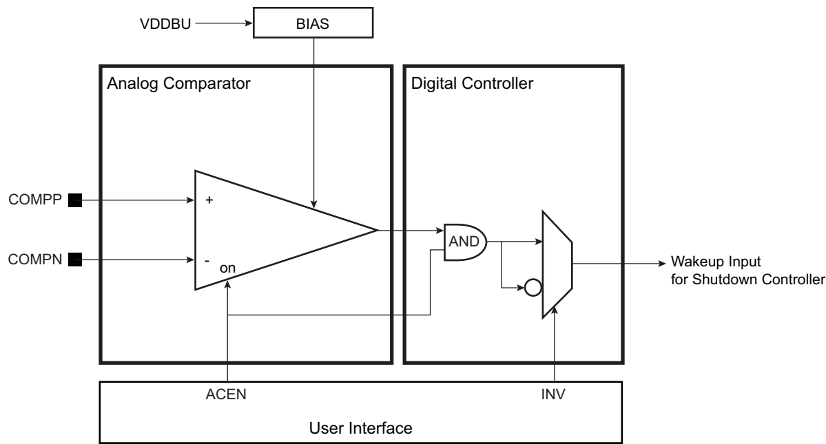
Figure 31-1: Analog Comparator Controller Block Diagram
