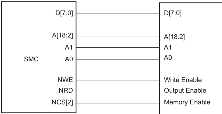
Figure 37-4: Memory Connection for an 8-bit Data Bus
