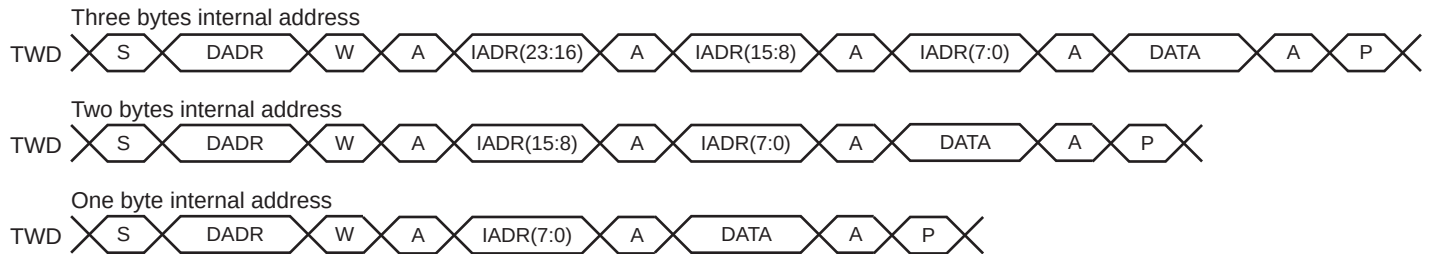
Figure 46-10: Master Write with One-, Two- or Three-Byte Internal Address and One Data Byte
