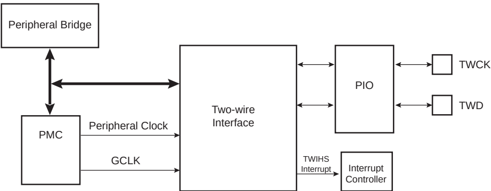
Figure 46-1: Block Diagram
