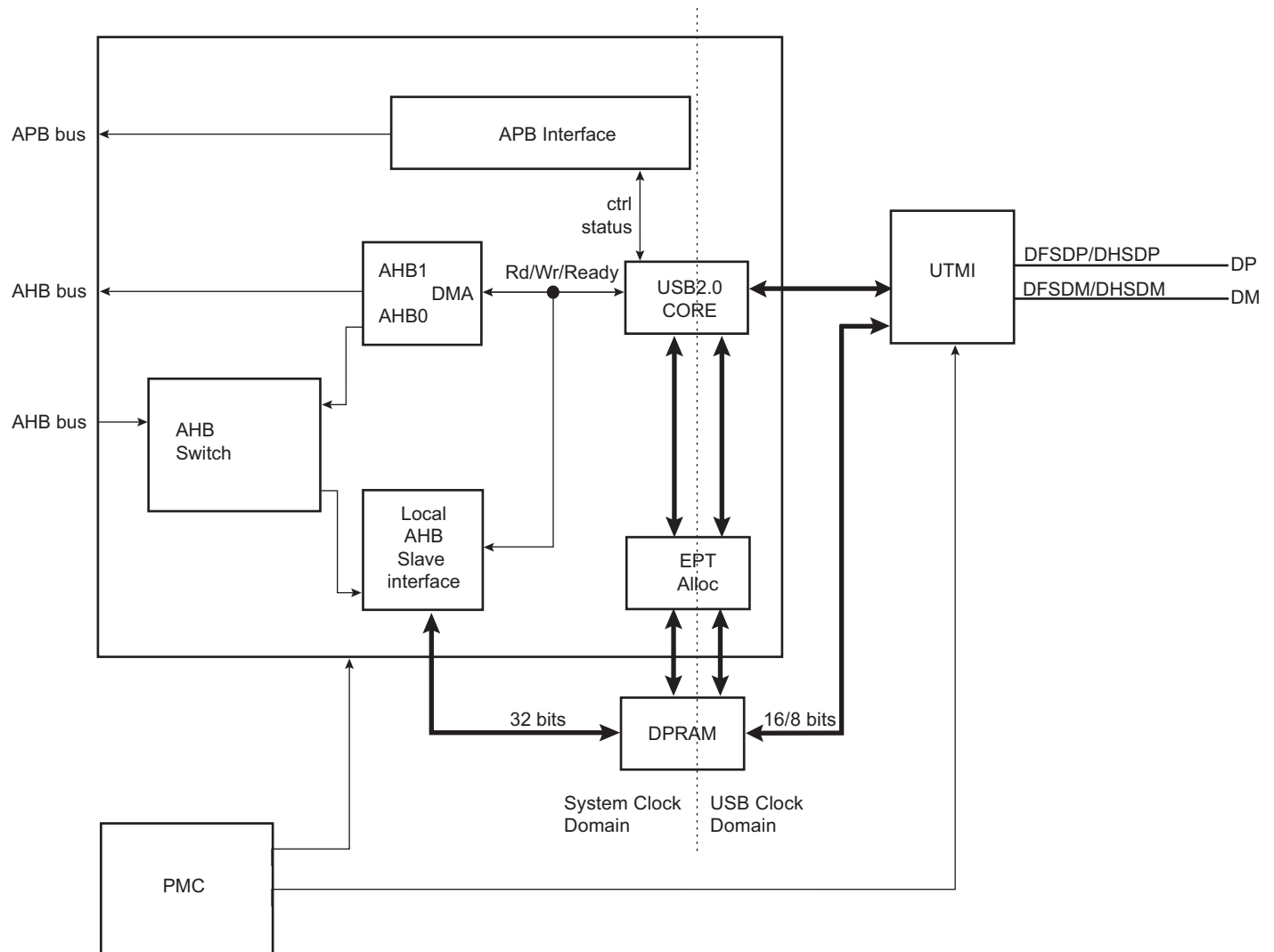
Figure 41-1: Block Diagram
