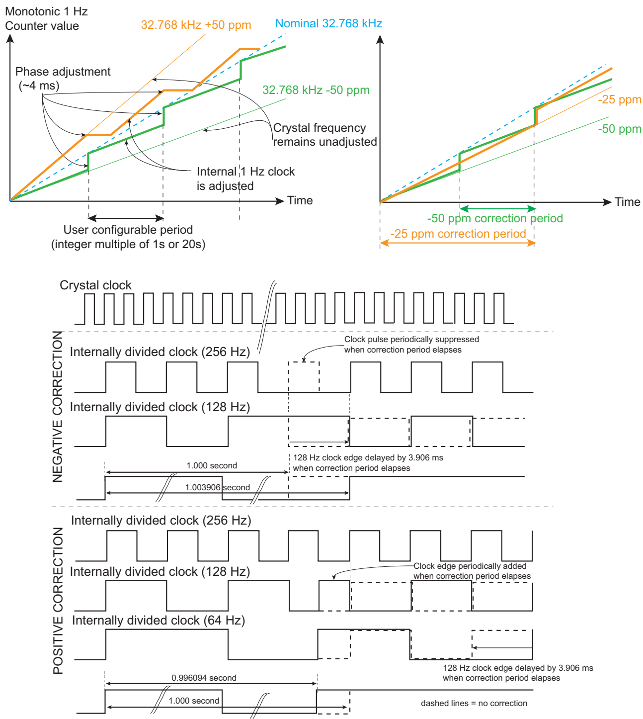
Figure 26-7: Calibration Circuitry Waveforms
