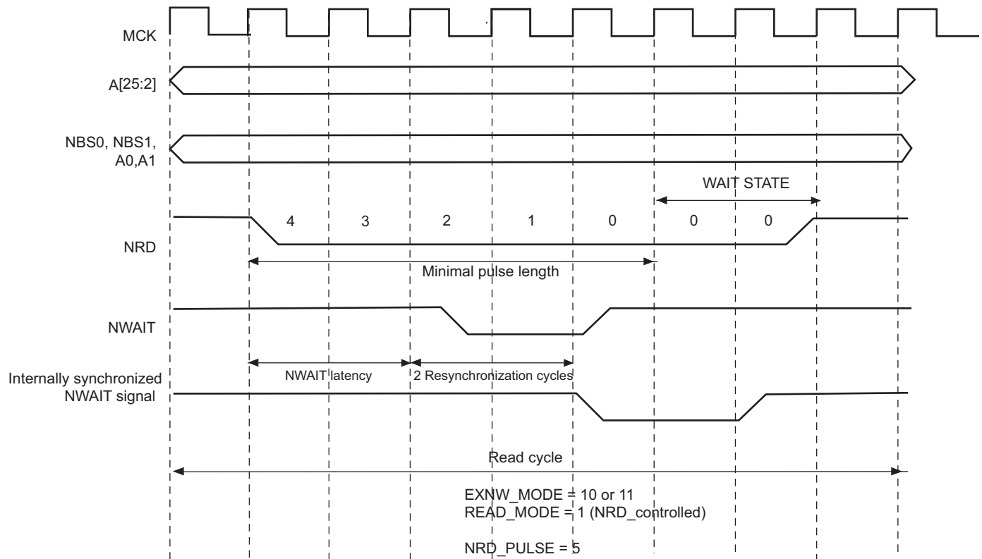
Figure 37-27: NWAIT Latency
