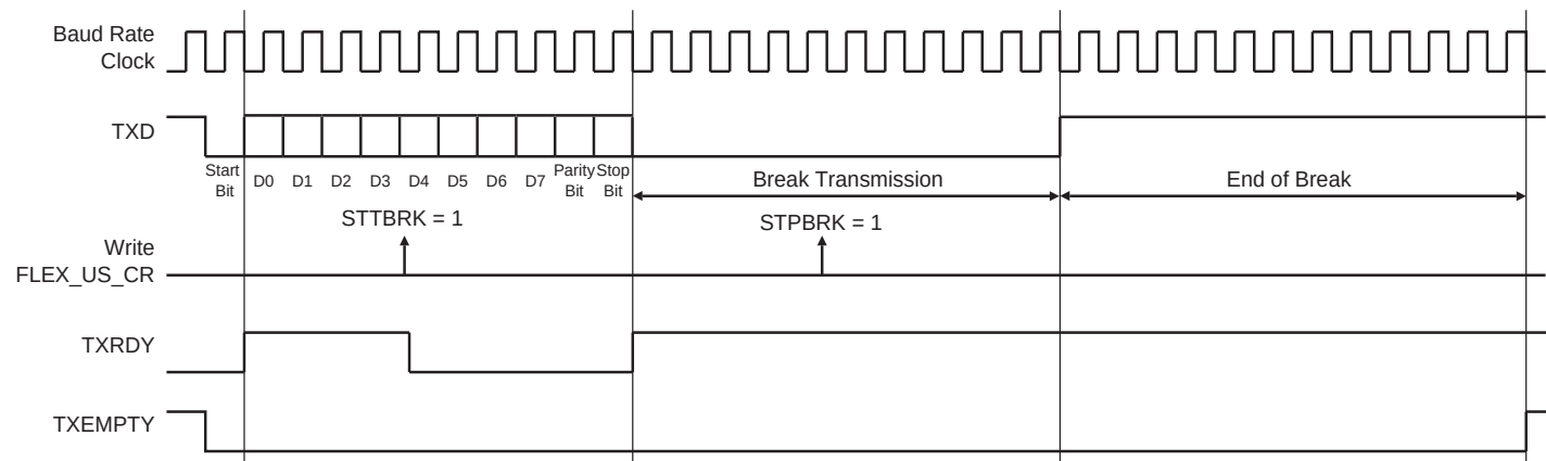
Figure 47-25: Break Transmission
