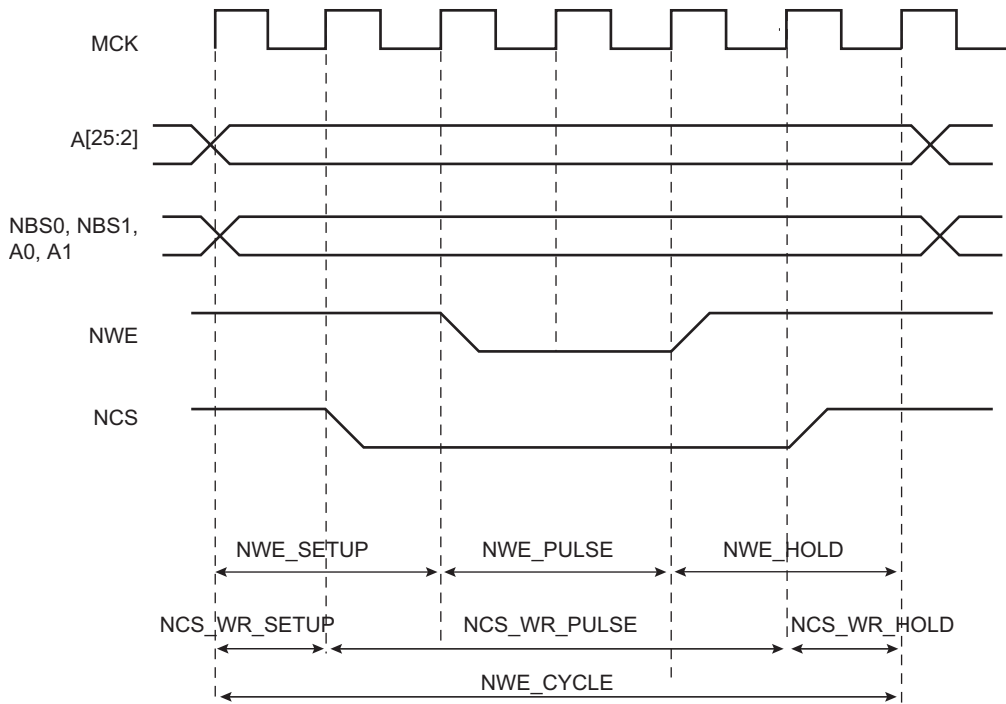
Figure 37-10: Write Cycle
