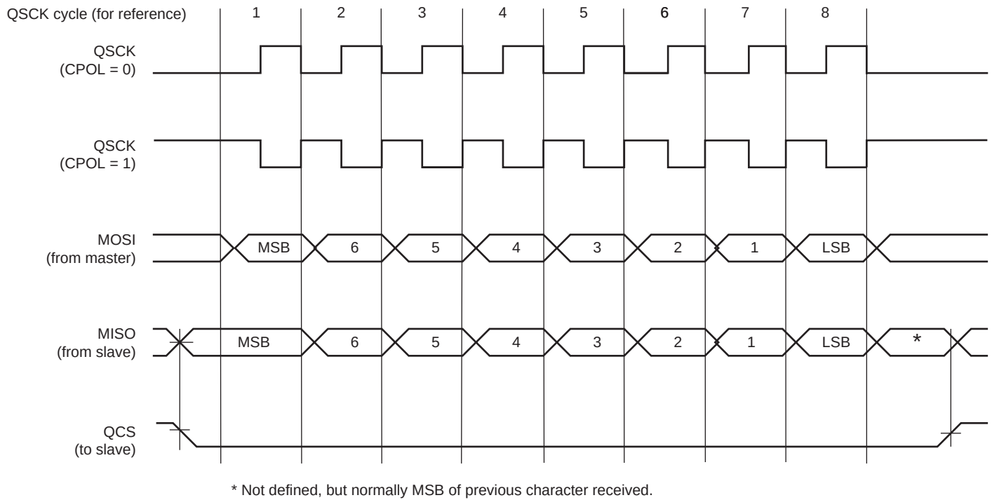
Figure 50-2: QSPI Transfer Format (QSPI_SCR.CPHA = 0, 8 bits per transfer)
