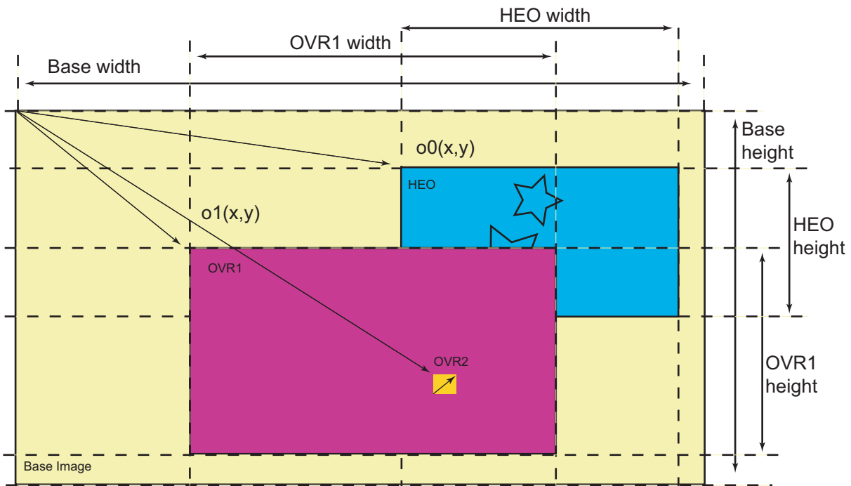
Figure 39-9: Overlay Example with Two Different Video Prioritization Algorithms
