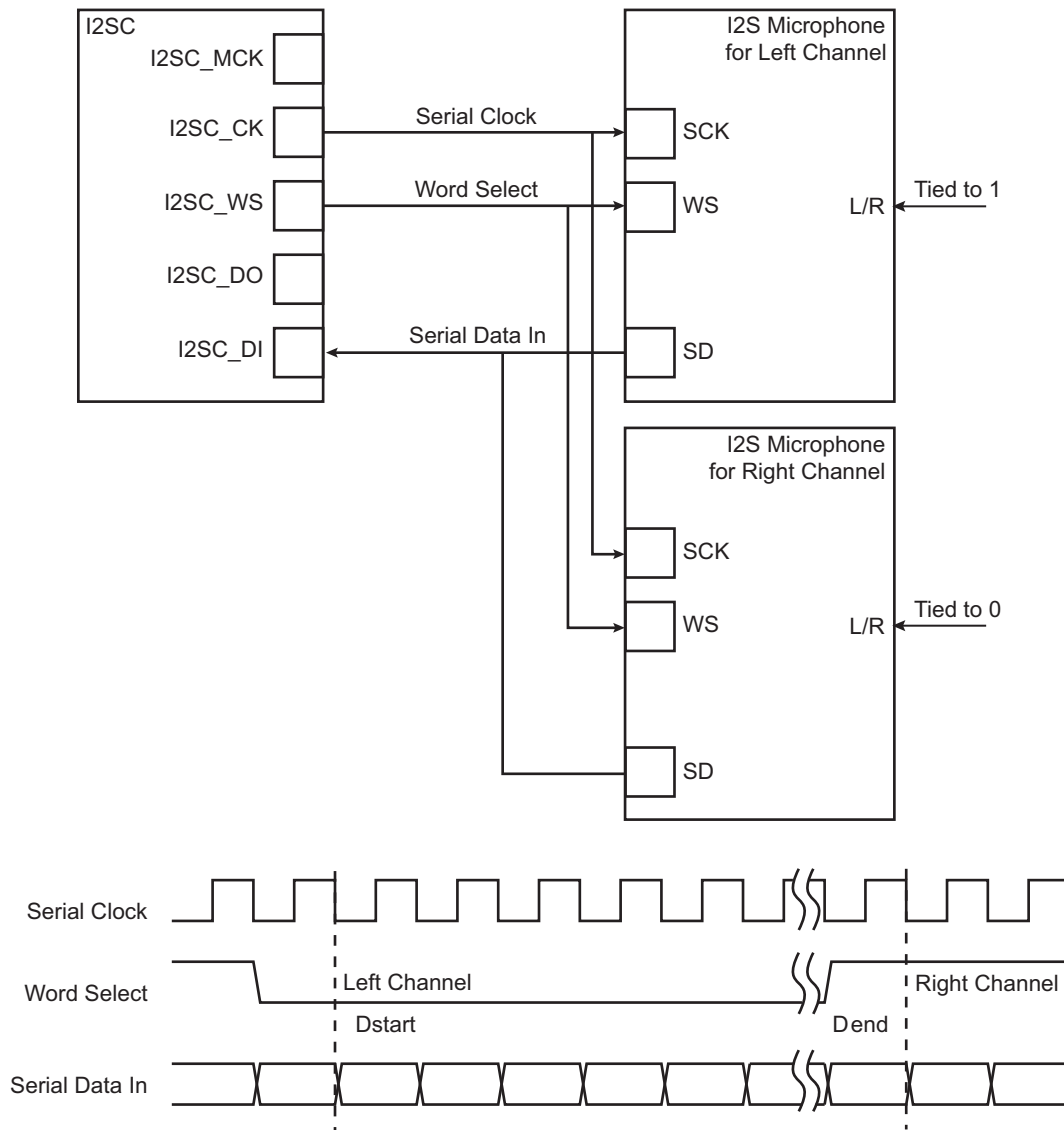
Figure 44-6: Dual Microphone Application Block Diagram
