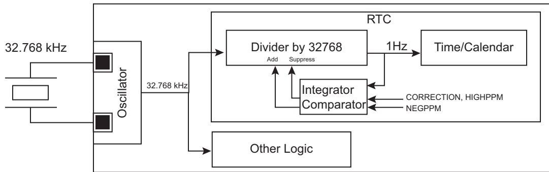
Figure 26-6: Calibration Circuitry
