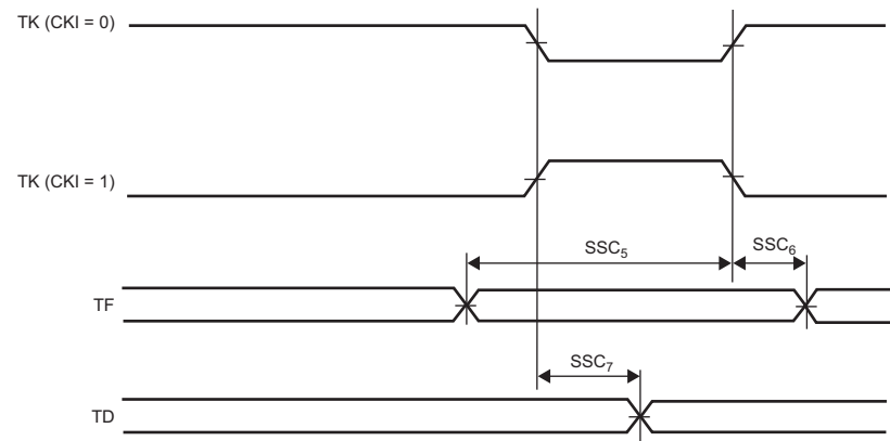
Figure 66-33: SSC Transmitter, TK and TF in Input
