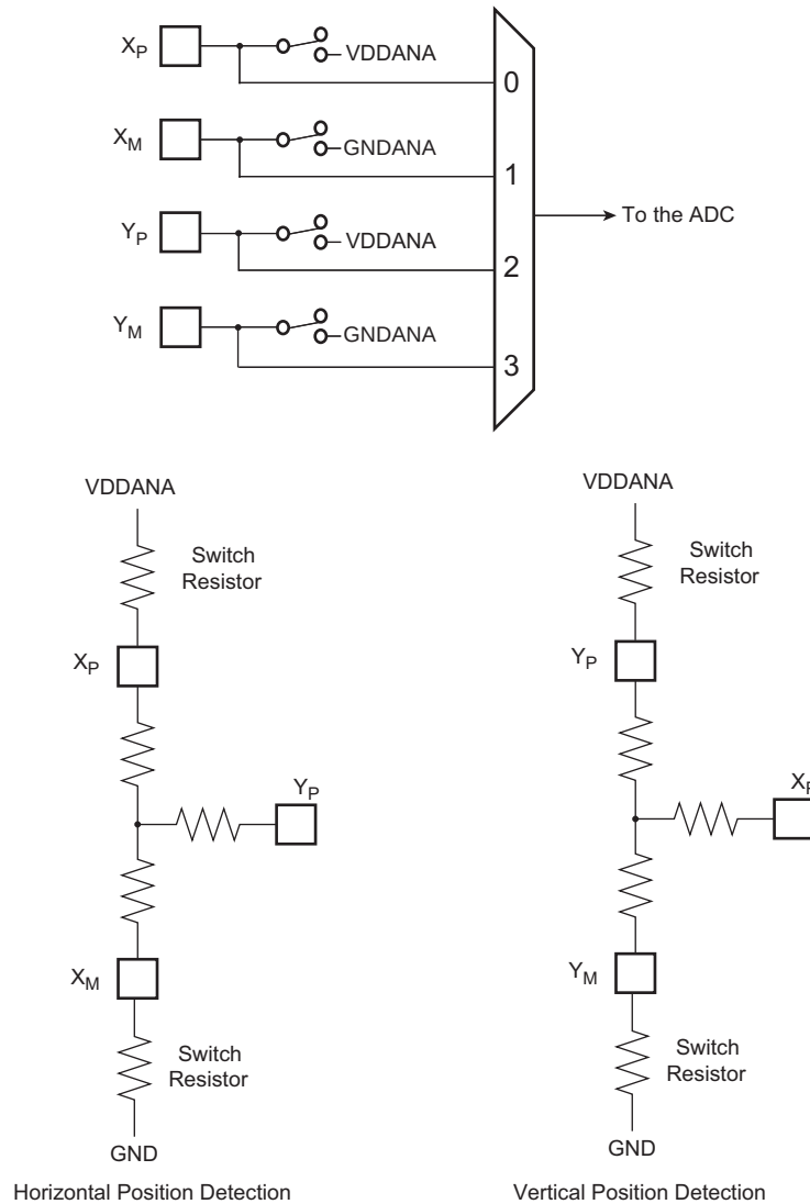
Figure 65-15: Touchscreen Switches Implementation
