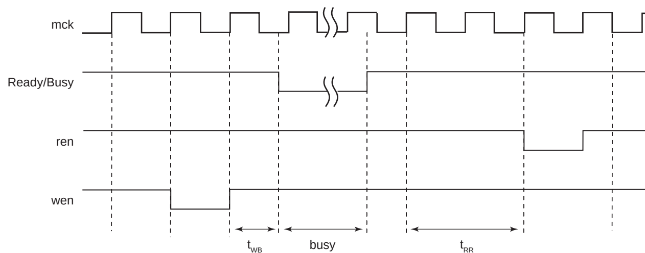
Figure 37-35: Ready/Busy Timing Configuration
