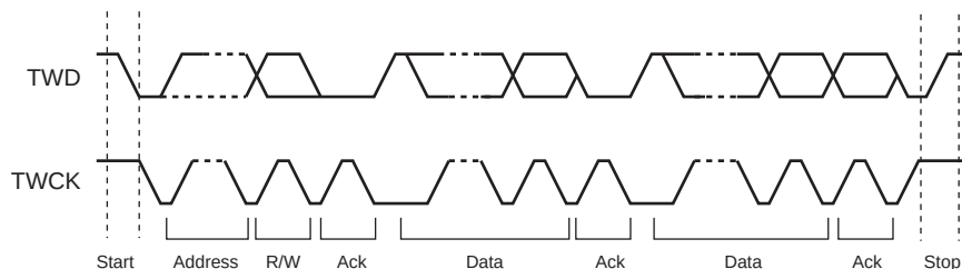
Figure 47-84: Transfer Format
