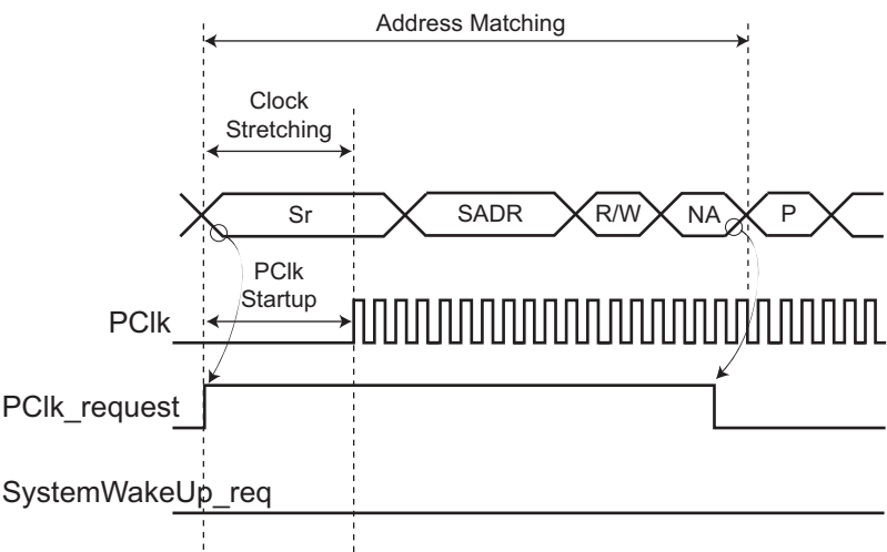
Figure 47-122: Address Does Not Match and Data Matching Disabled
