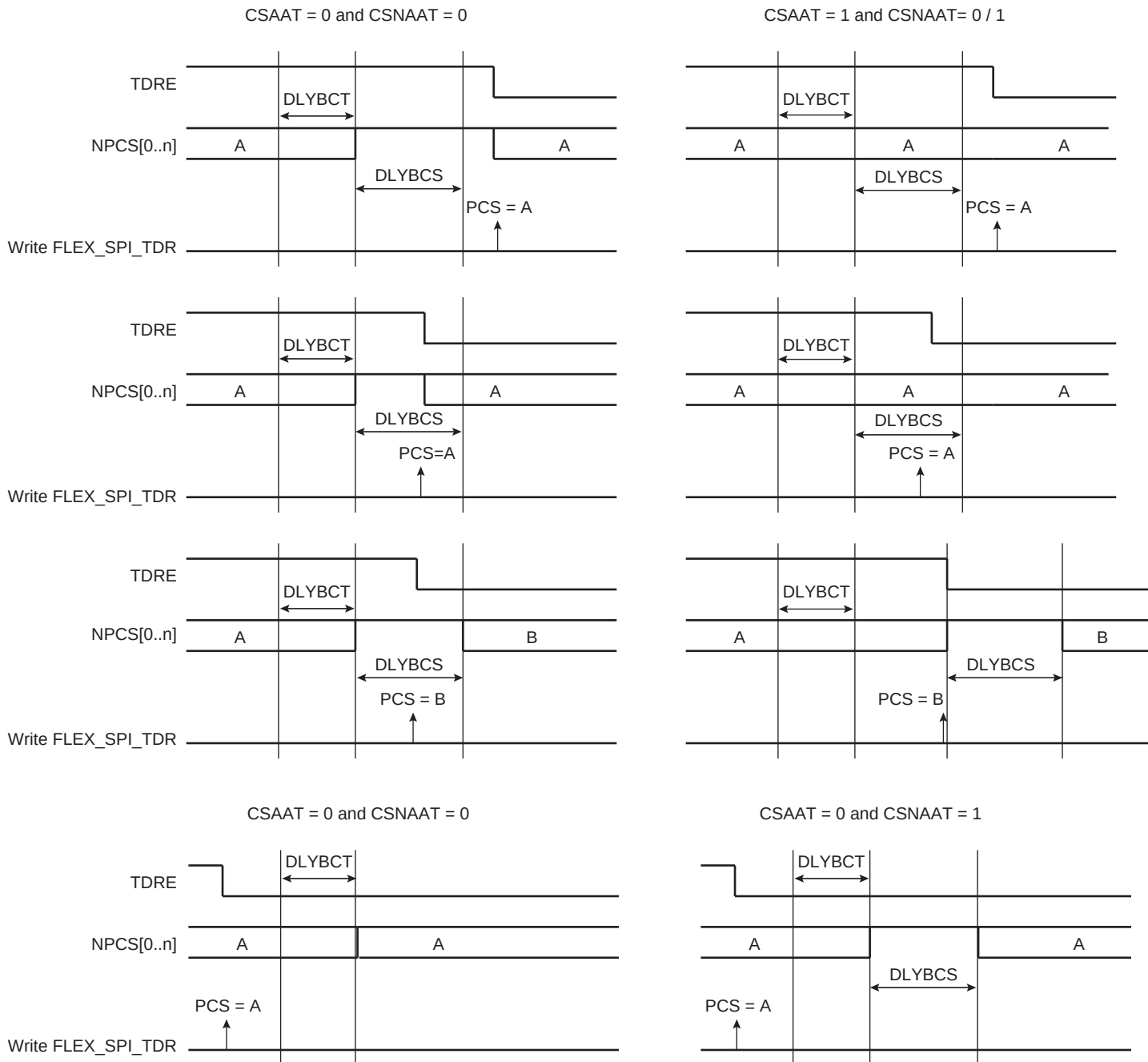
Figure 47-73: Peripheral Deselection
