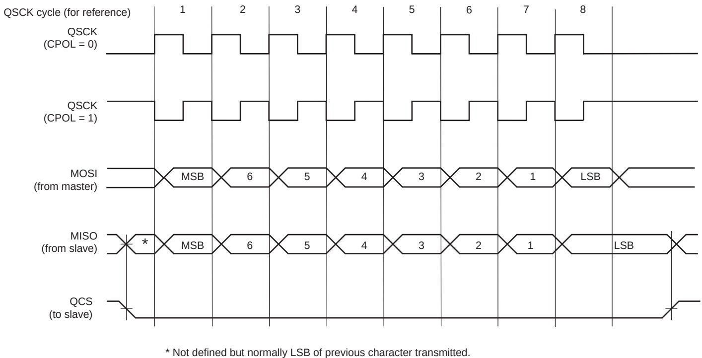
Figure 50-3: QSPI Transfer Format (QSPI_SCR.CPHA = 1, 8 bits per transfer)
