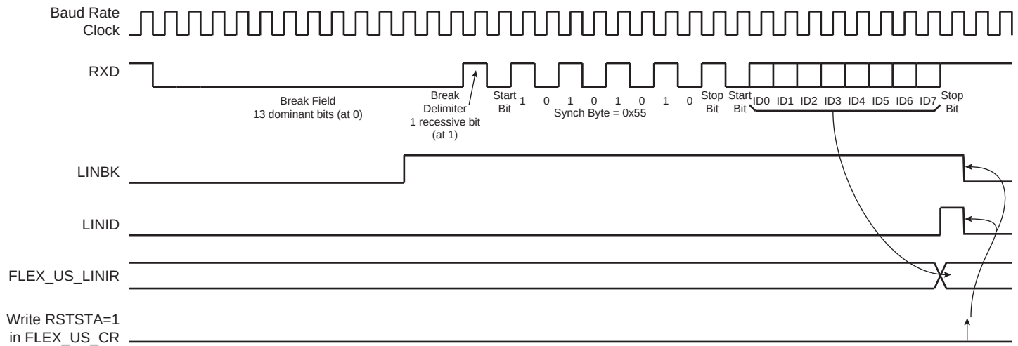
Figure 47-42: Header Reception
