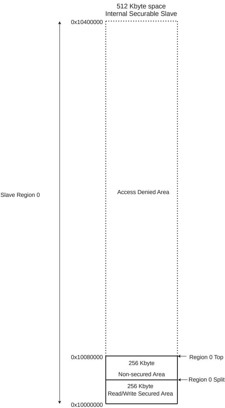
Figure 18-2: Partitioning Example of an Internal Securable Slave Featuring 1 Security Region of 512 Kbytes Split into 1 or 2 Security Areas of 4 Kbytes to 512 Kbytes
