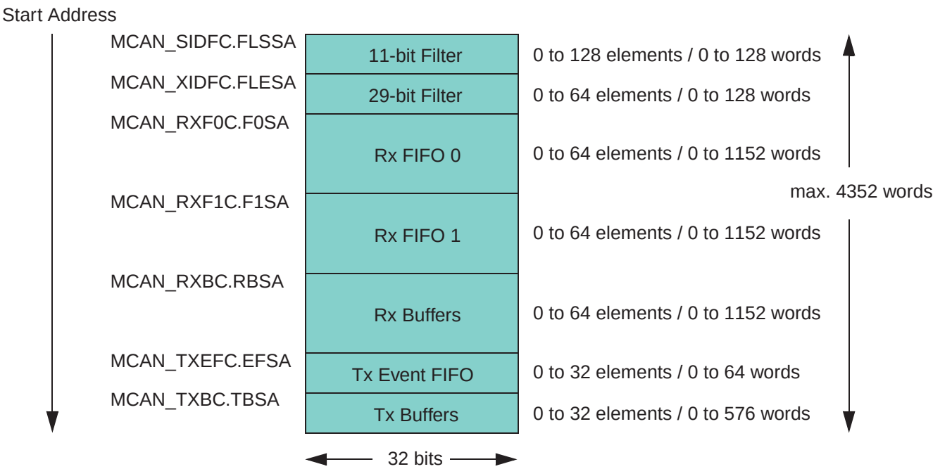
Figure 53-12: Message RAM Configuration
