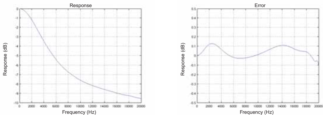
Figure 43-9: De-emphasis Filter: Frequency Response & Error ( f_s = 44.1 kHz)
