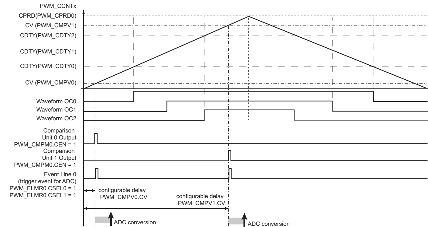
Figure 56-26: Event Line Generation Waveform (Example)
