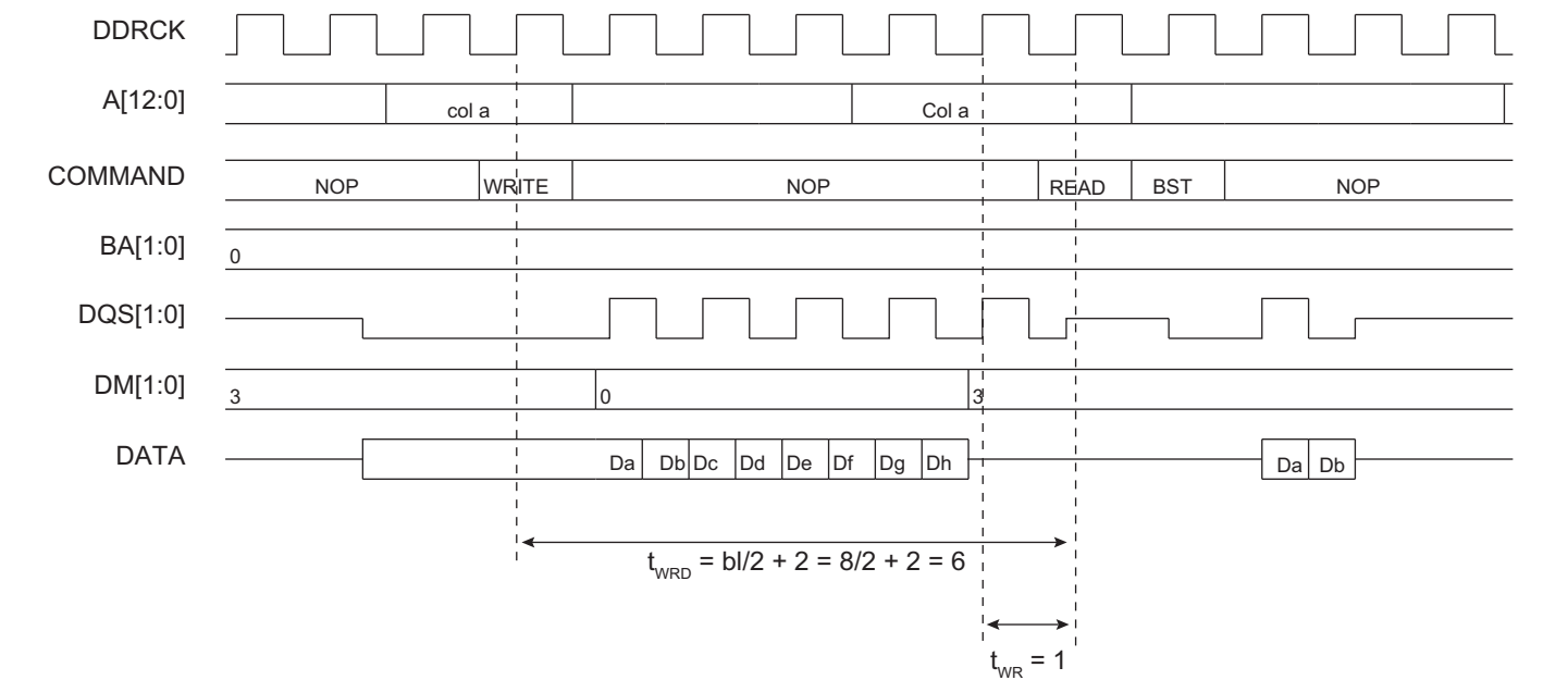
Figure 36-6: Write Command Followed by a Read Command without Burst Write Interrupt, DDR-SDRAM Devices
