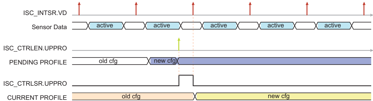
Figure 52-18: Update Profile Timing Diagram
