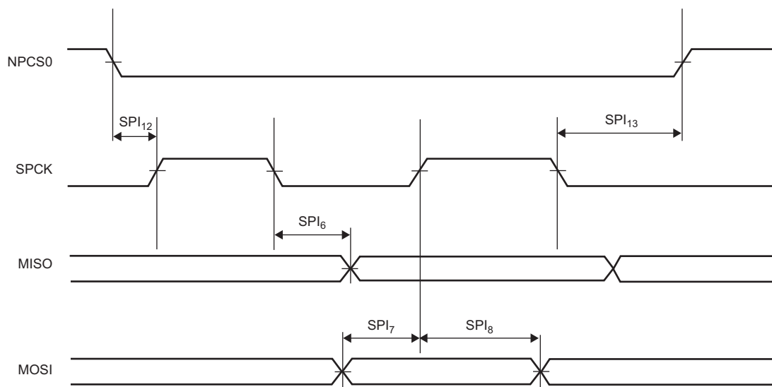
Figure 66-21: SPI Slave Modes 0 and 3
