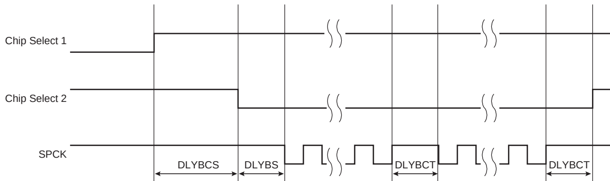
Figure 47-71: Programmable Delays
