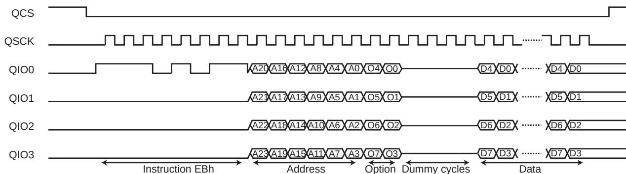
Figure 50-8: Instruction Frame
