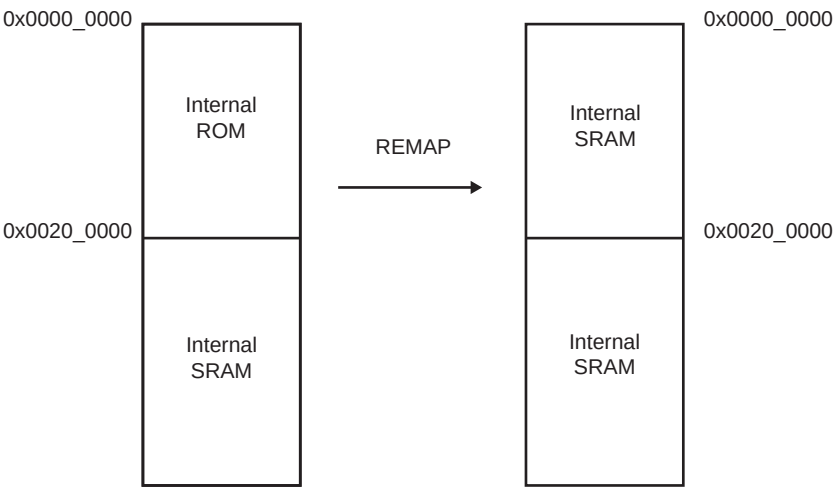
Figure 16-6: Remap Action after Download Completion
