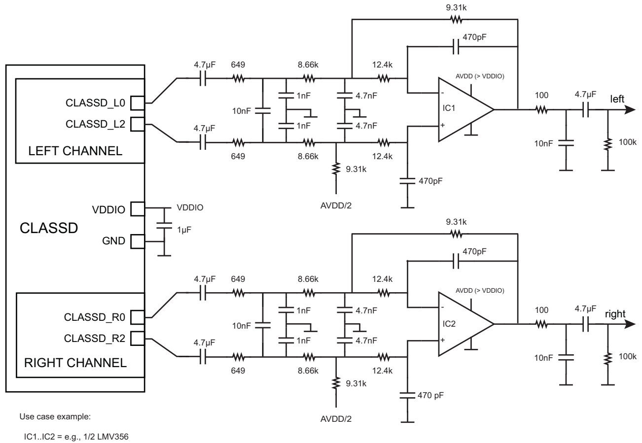
Figure 43-17: Use Case 3A: Stereo Audio DAC With Active Low Pass Filter and Single-ended Outputs
