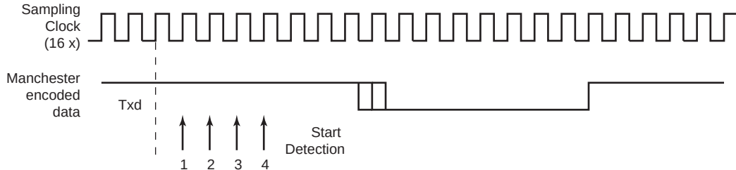
Figure 47-13: Asynchronous Start Bit Detection
