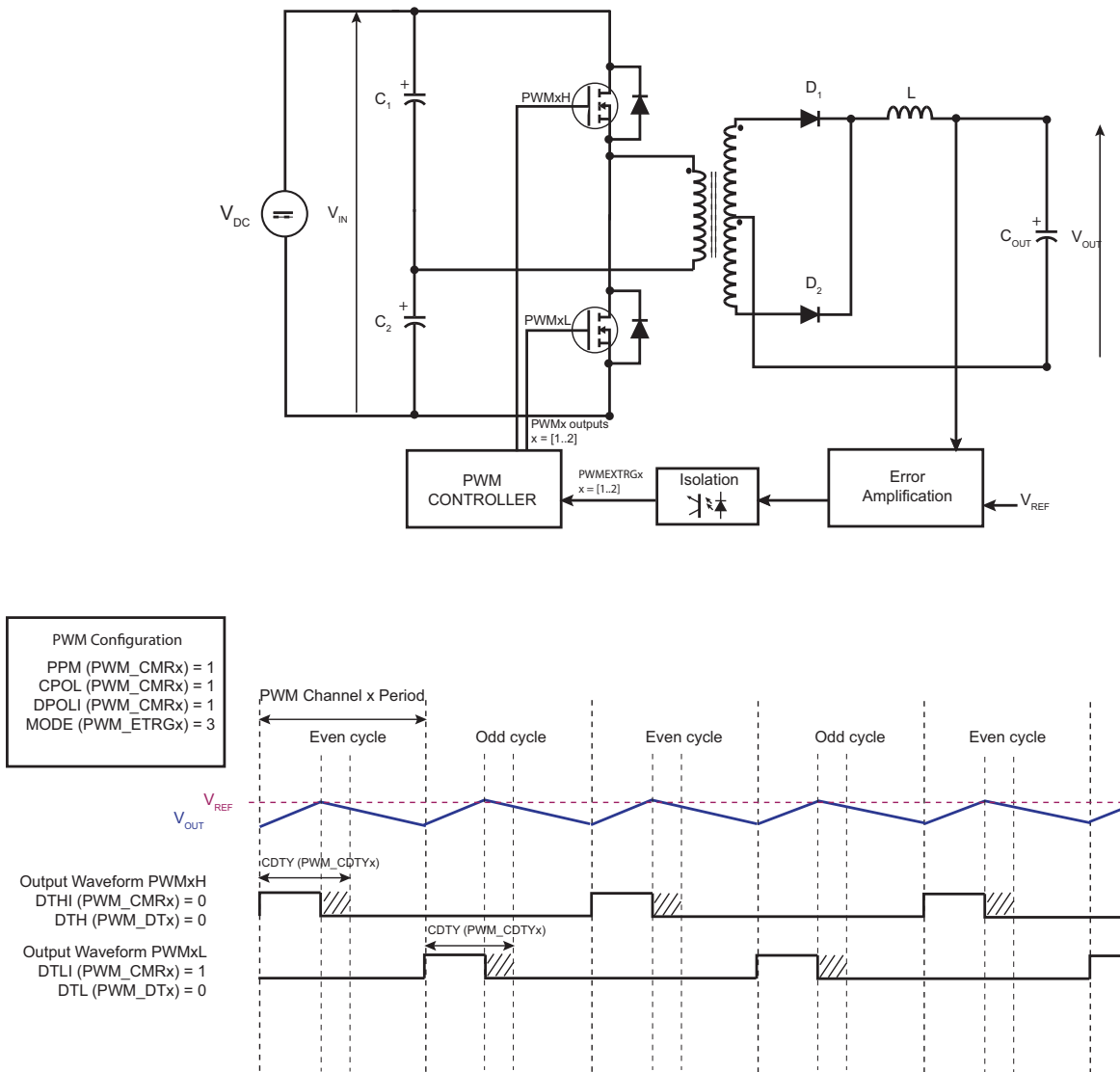
Figure 56-14: Half-Bridge Converter Application: Feedback Regulation
