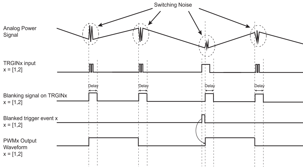
Figure 56-33: Leading-Edge Blanking
