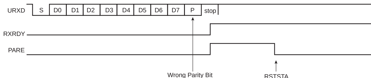
Figure 48-7: Parity Error
