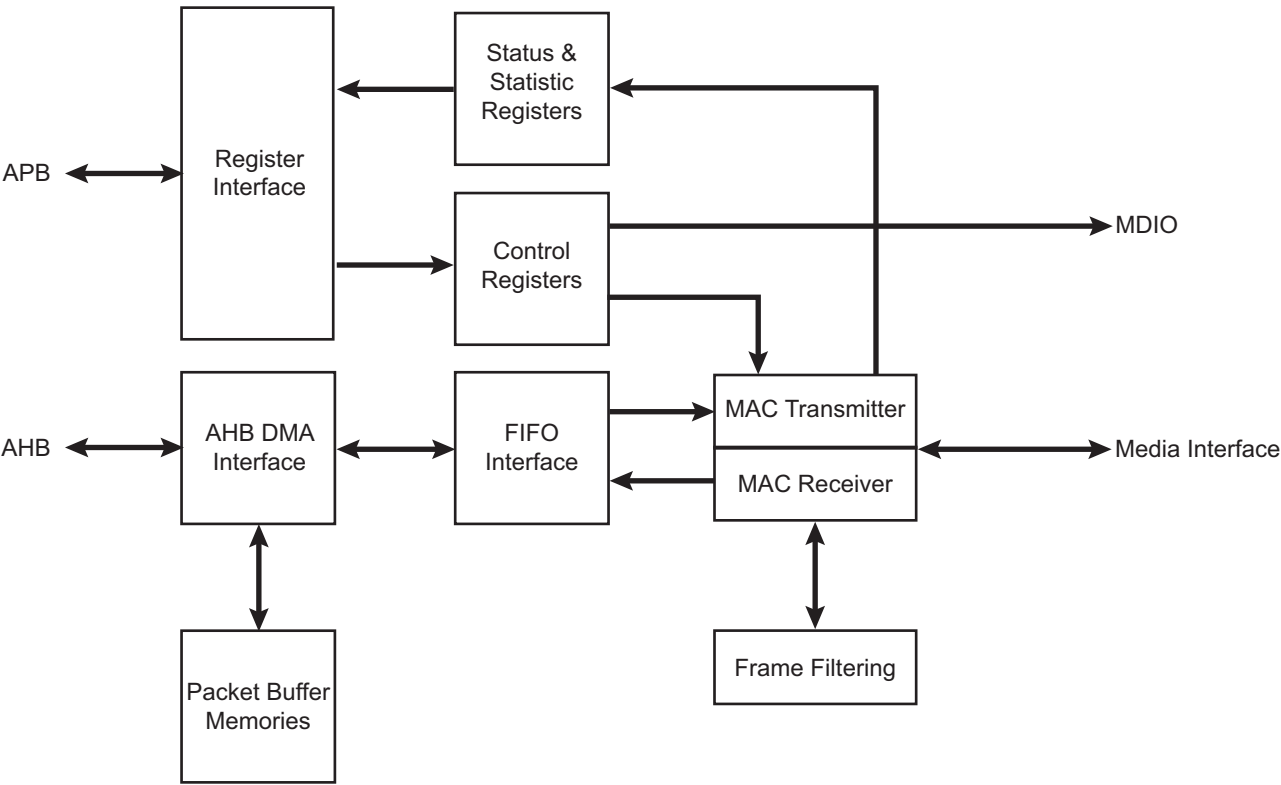
Figure 40-1: Block Diagram
