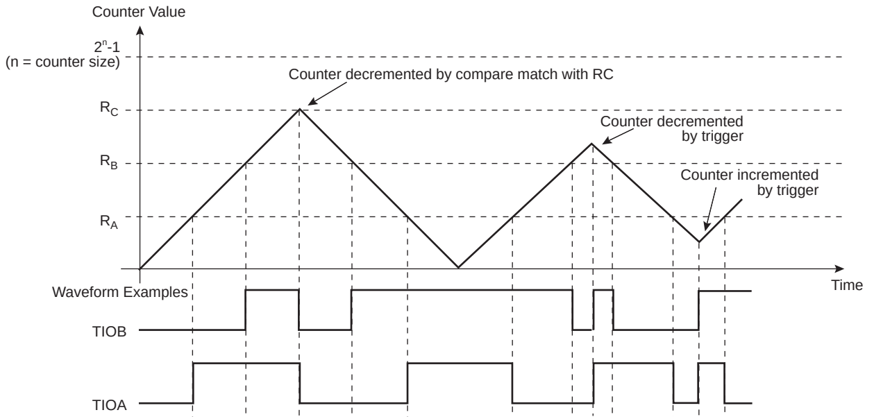
Figure 54-15: WAVSEL = 11 with Trigger
