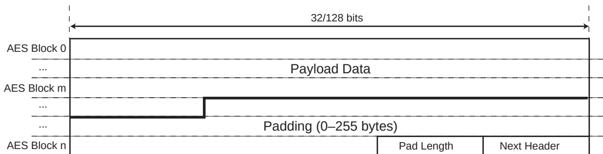
Figure 60-9: IPSEC Padding
