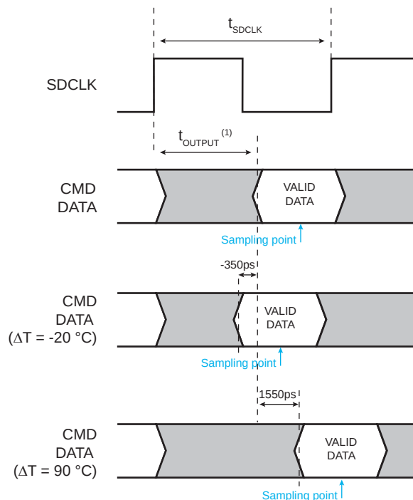
Figure 51-5: Temperature Effect on Data Window
