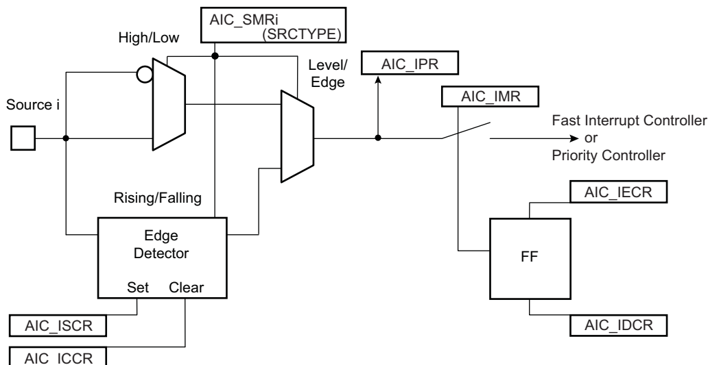
Figure 21-5: External Interrupt Source Input Stage
