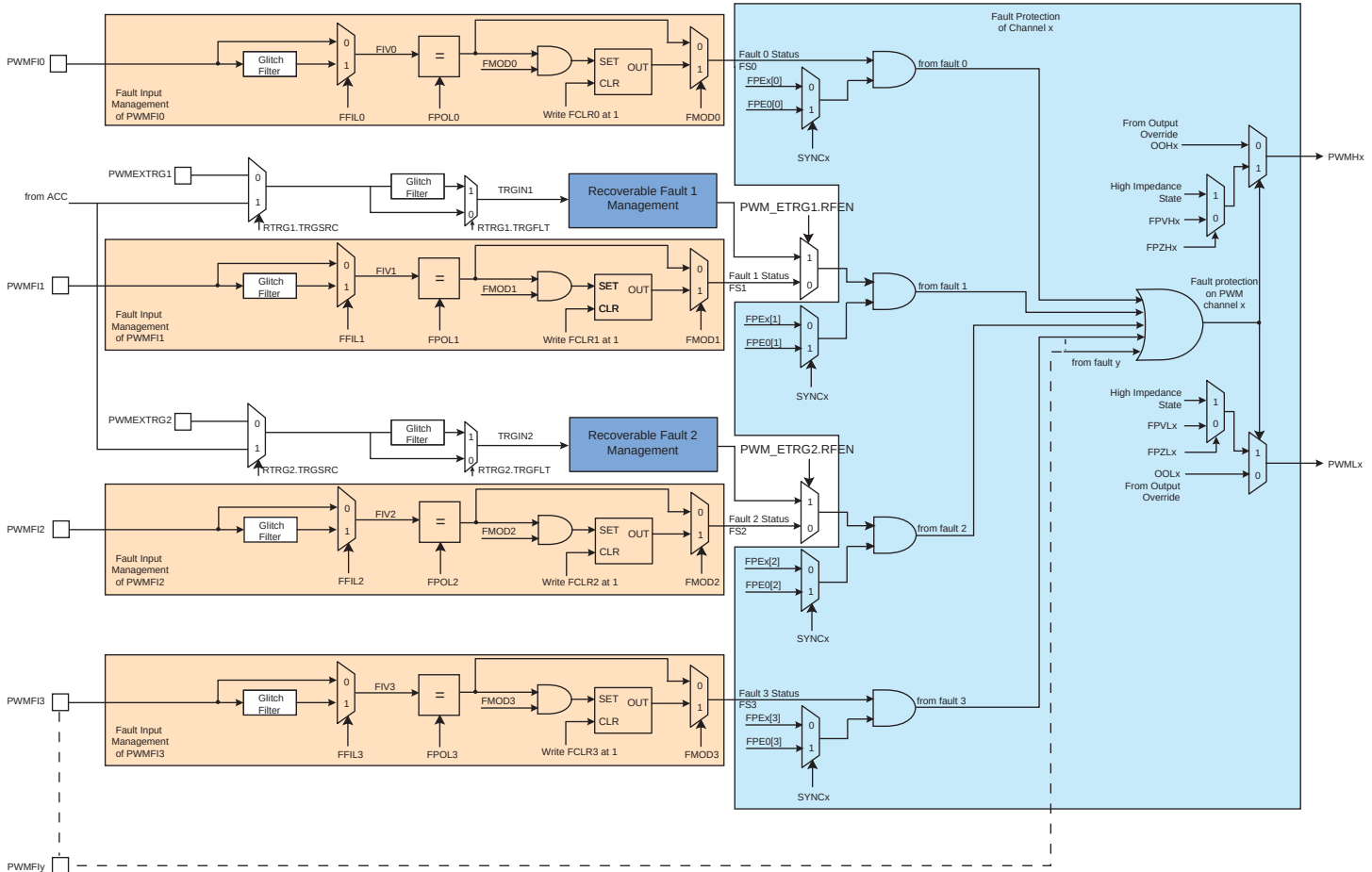
Figure 56-16: Fault Protection
