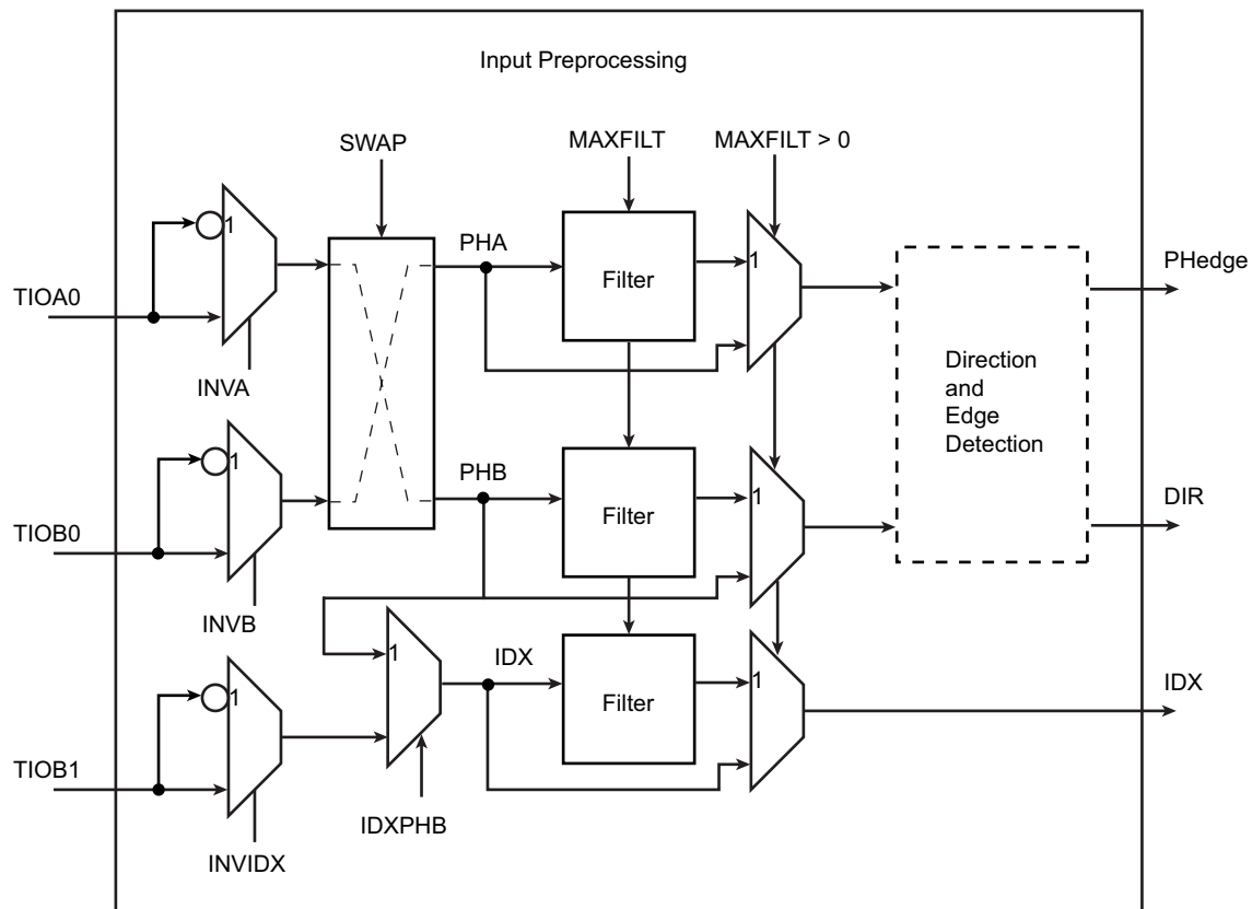
Figure 54-18: Input Stage
