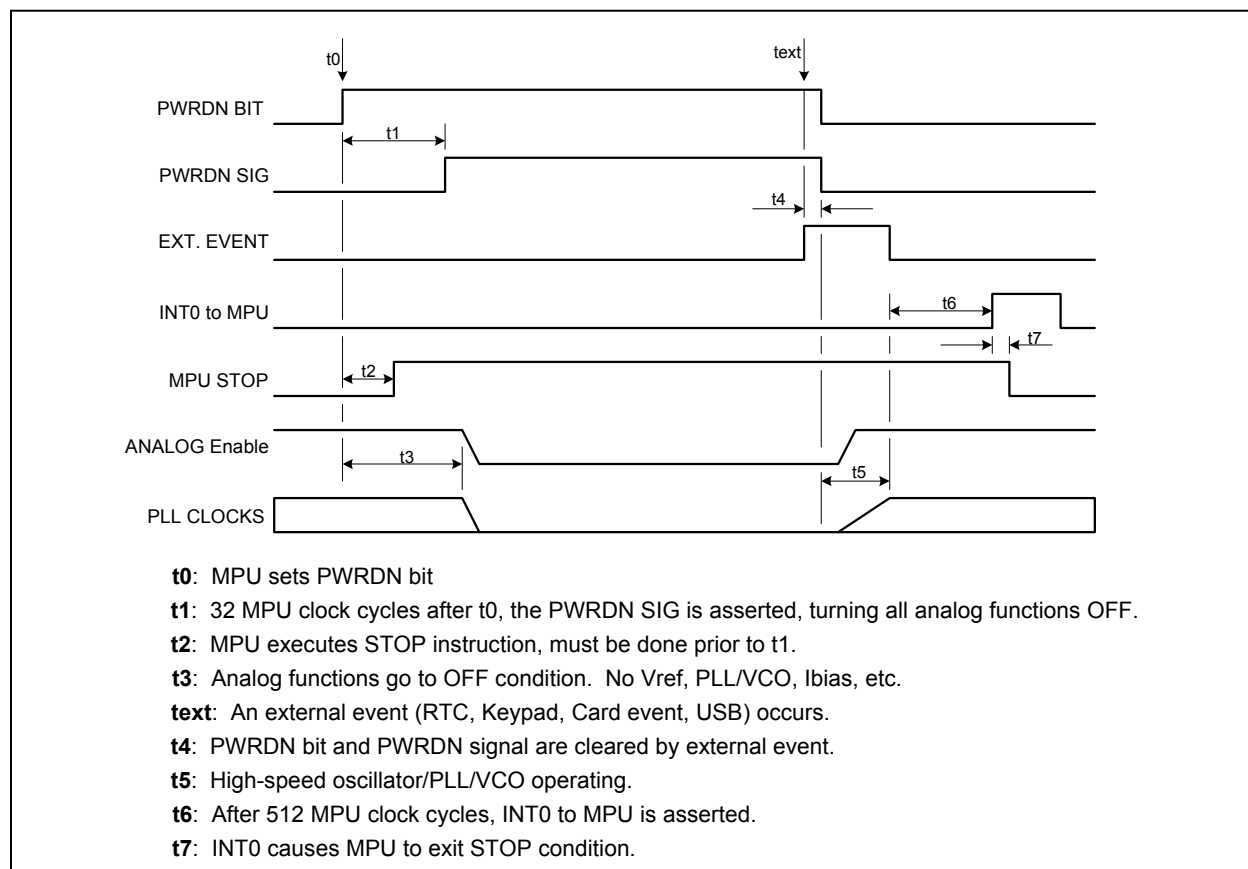
Figure 8: Power-Down Sequencing
