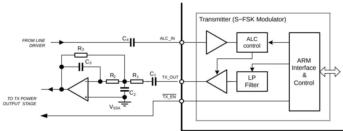
Figure 7. TX_OUT Filter
