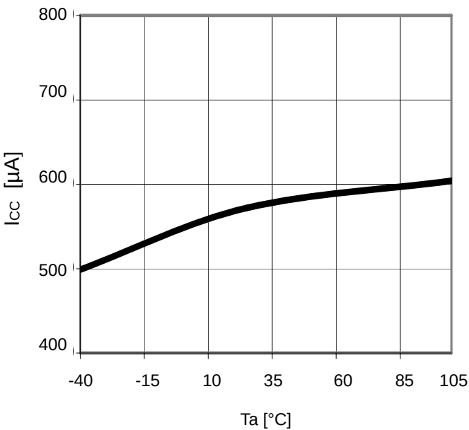
Figure 22. T_a - I_{cc}
