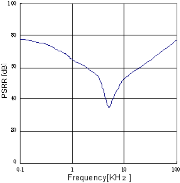
Figure 32. PSRR (Io=0mA)
