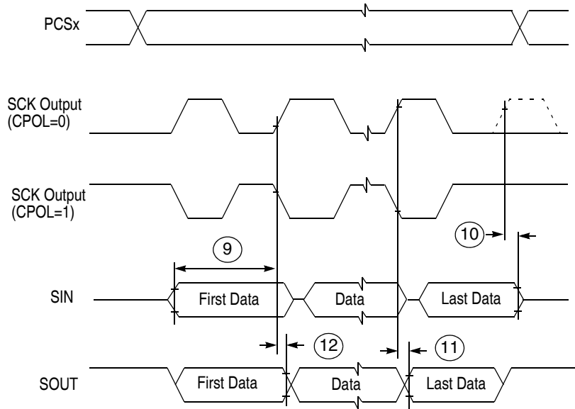
Figure 23. DSPI Modified Transfer Format Timing — Master, CPHA = 1
