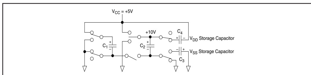
Figure 21. Charge Pump - Phase 4
