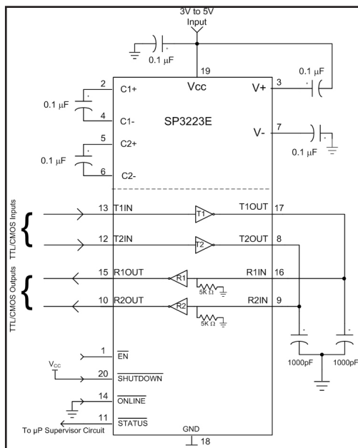
Figure 14. Loopback Test Circuit for RS-232 Driver Data Transmission Rates
