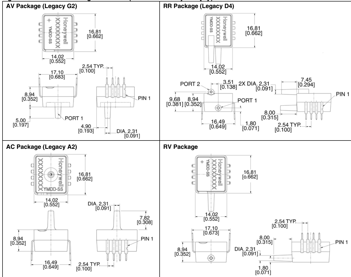
Figure 4. Dimensional Drawings and Pinout (For reference only: mm [in].)
