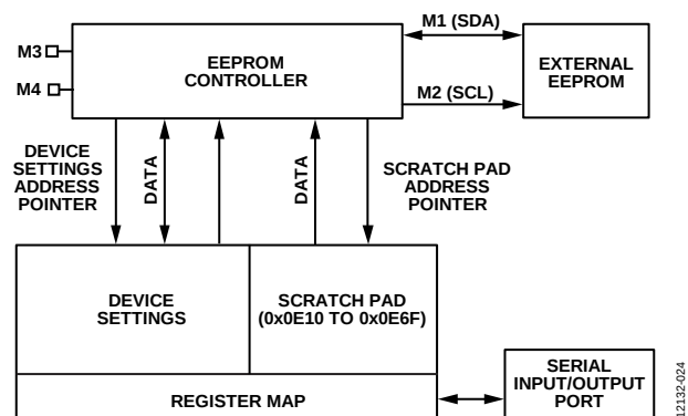
Figure 32. EEPROM Functional Diagram
