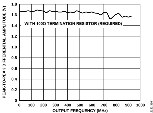
Figure 10. Peak-to-Peak Differential Amplitude vs. Output Frequency, 28 mA Mode (LVPECL-Compatible Mode) with 100Ω Termination Resistor (Required)
