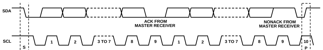
Figure 43. Data Transfer Process (Master Read Mode, 2-Byte Transfer), First ACK From Slave
