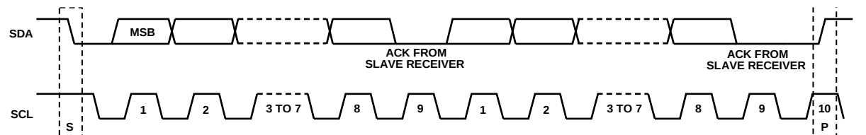
Figure 42. Data Transfer Process (Master Write Mode, 2-Byte Transfer)
