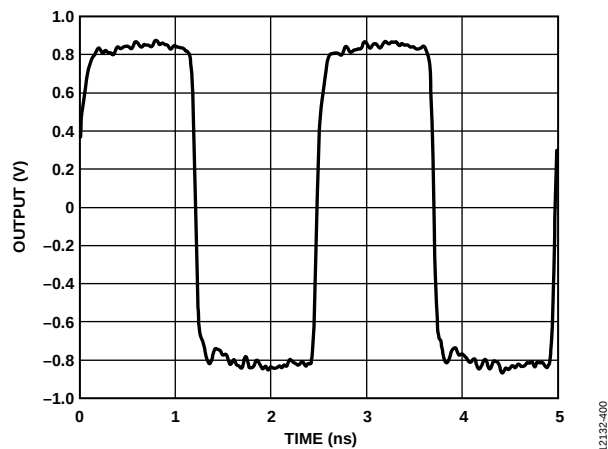
Figure 14. Output Waveform, 28 mA LVPECL-Compatible Mode (400 MHz) with 100Ω Termination Resistor
