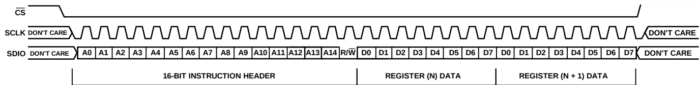
Figure 37. Serial Control Port Write—LSB First, Address Increment, Two Bytes of Data
