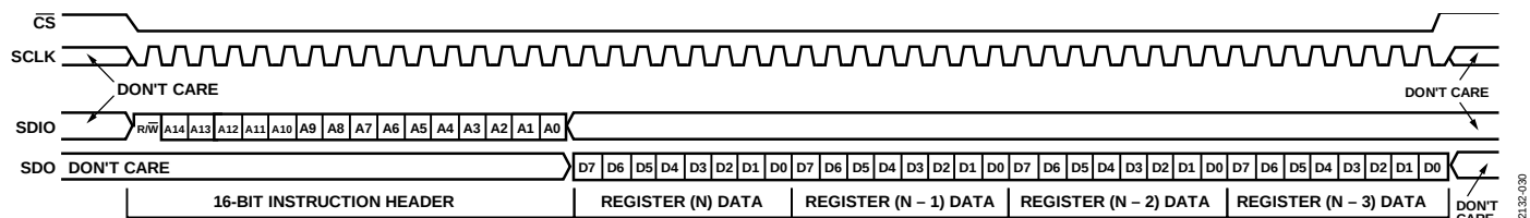
Figure 34. Serial Control Port Read—MSB First, Address Decrement, Four Bytes of Data
