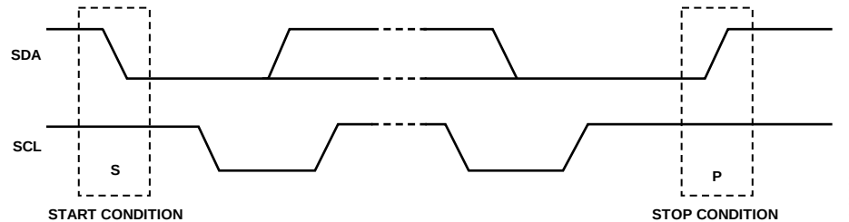
Figure 40. Start and Stop Conditions
