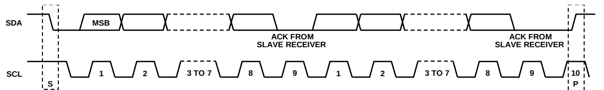
Figure 41. Acknowledge Bit
