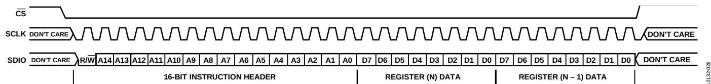
Figure 33. Serial Control Port Write—MSB First, Address Decrement, Two Bytes of Data
