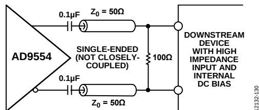
Figure 21. Destination Self-Biased Differential Receiver; Use 14 mA Mode for LVDS-Compatible Amplitude or 28 mA for LVPECL-Compatible Amplitudes (100 \Omega resistor must be as close to the destination receiver as possible.)
