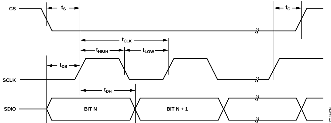
Figure 38. Serial Control Port Timing—Write
