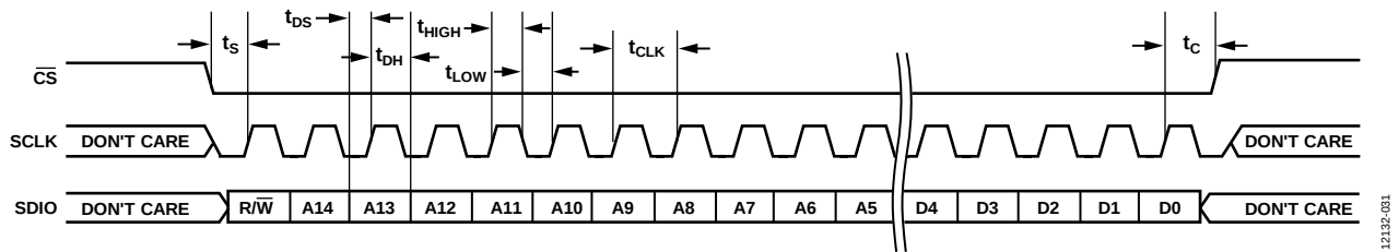
Figure 35. Timing Diagram for Serial Control Port Write—MSB First
