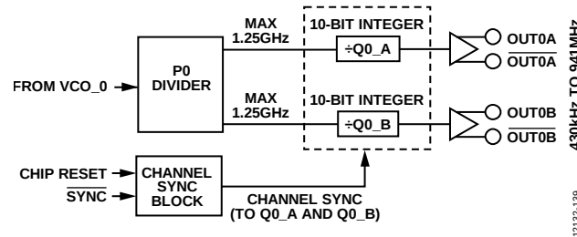
Figure 31. Clock Distribution Block Diagram from VCO_0 for the PLL_0
