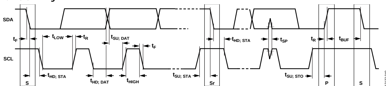
Figure 44. I 2 C Serial Port Timing
