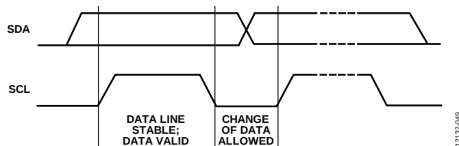
Figure 39. Valid Bit Transfer
