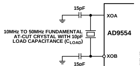
Figure 24. System Clock Input (XOA/XOB) in Crystal Mode (The capacitor values shown are for a crystal with a C_{LOAD} = 10 pF. The values of 15 pF shunt capacitors shown here must equal 2 \times (C_{LOAD} - C_{STRAY}) , where C_{STRAY} is typically 2 pF to 5 pF.)
