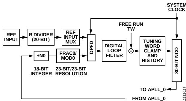
Figure 27. DPLL_0 Core
