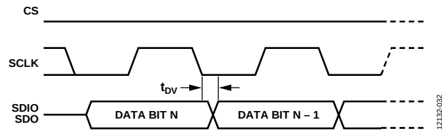
Figure 36. Timing Diagram for Serial Control Port Register Read—MSB First
