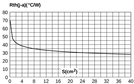
Fig. 8: Thermal resistance junction to ambient versus copper surface under tab (Epoxy printed circuit board FR4, copper thickness: 35 \mu m) (D²PAK).
