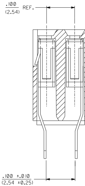
SECTION E-E
