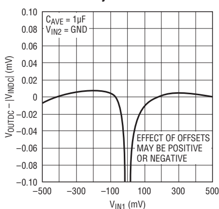
DC Linearity
