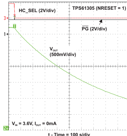
Figure 86. Shutdown (HC_SEL = 1)
