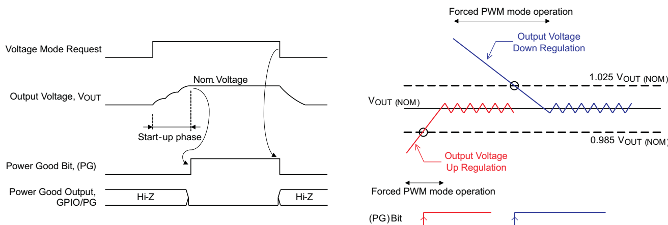
Figure 37. Power Good Operation (DIR = 1, GIPIOTYPE = 1)
