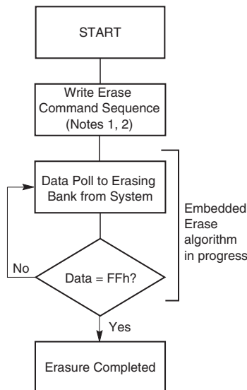
Figure 15.2 Erase Operation
