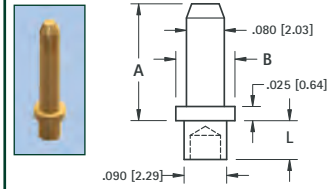
.080 (2.0) PIN - SWAGE MOUNT
