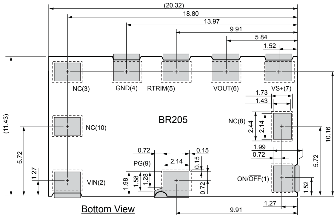
PCB Board Layout and Pin-out Diagram
