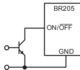
Figure 5. \text{ON}/\overline{\text{OFF}} peripheral circuit
