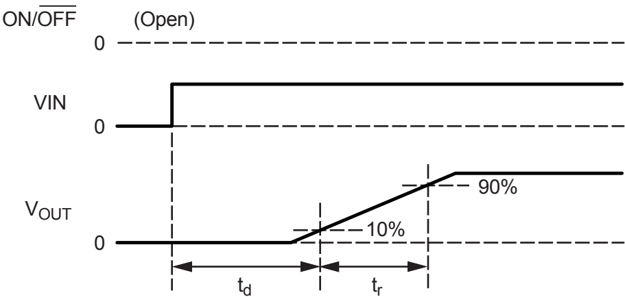
Figure 1. Start Delay Time, t_d , definition
