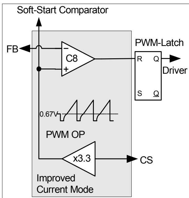
Figure 4 Current Mode
