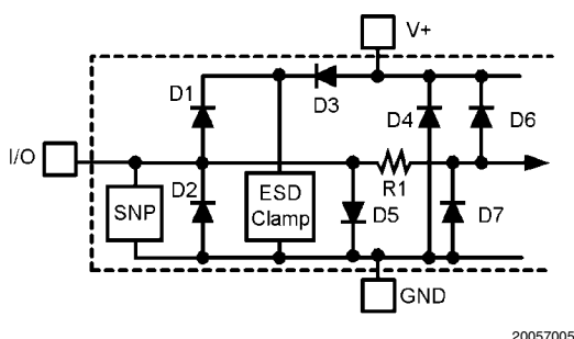
FIGURE 1. ESD Protection Input Structure
