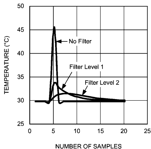
FIGURE 7. Impulse Response of the Digital Filter
