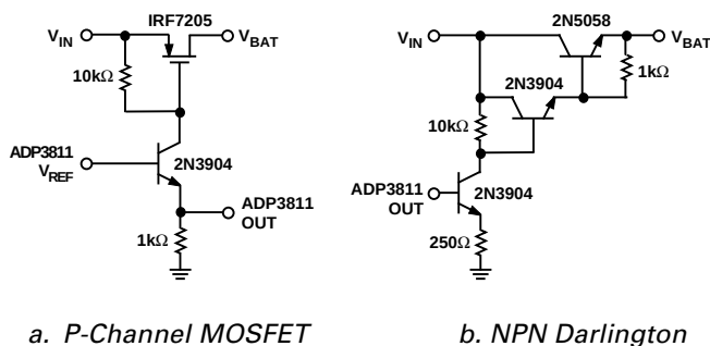
Figure 30. Alternative Pass Transistor for Linear Regulator realizations of the pass element are shown in Figure 30. In case (a), the pass transistor is a P-channel MOSFET. This provides a lower dropout voltage so that V_{BAT} can be within a few hundred millivolts of V_{IN} . In case (b), a Darlington configuration of two npn transistors is used. The dropout voltage of this circuit is approximately 2 V for a 0.5 A charge current.
