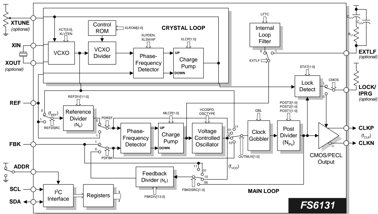
Figure 2: Block Diagram
