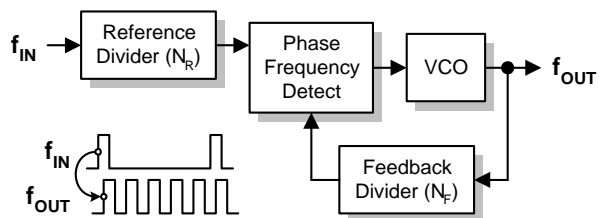
Figure 5: Simple PLL
