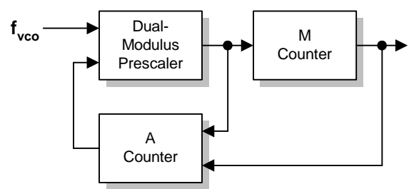
Figure 3: Feedback Divider
