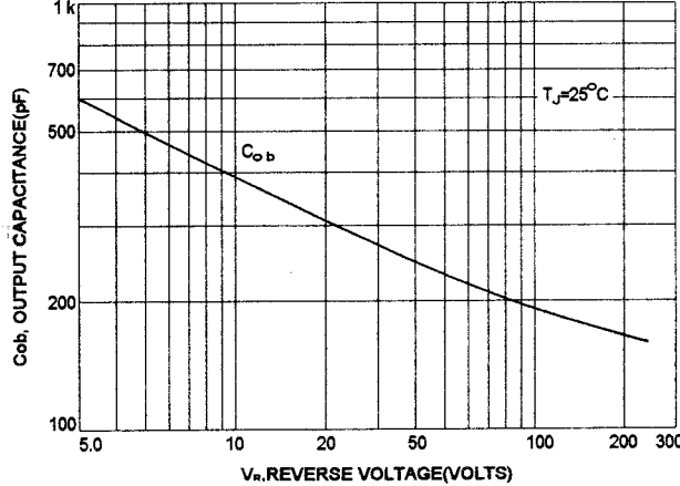
OUTPUT CAPACITANCES
