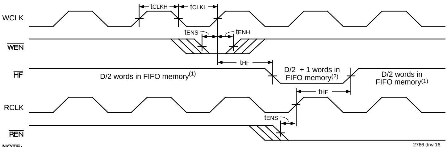
Figure 14. Half-Full Flag Timing
