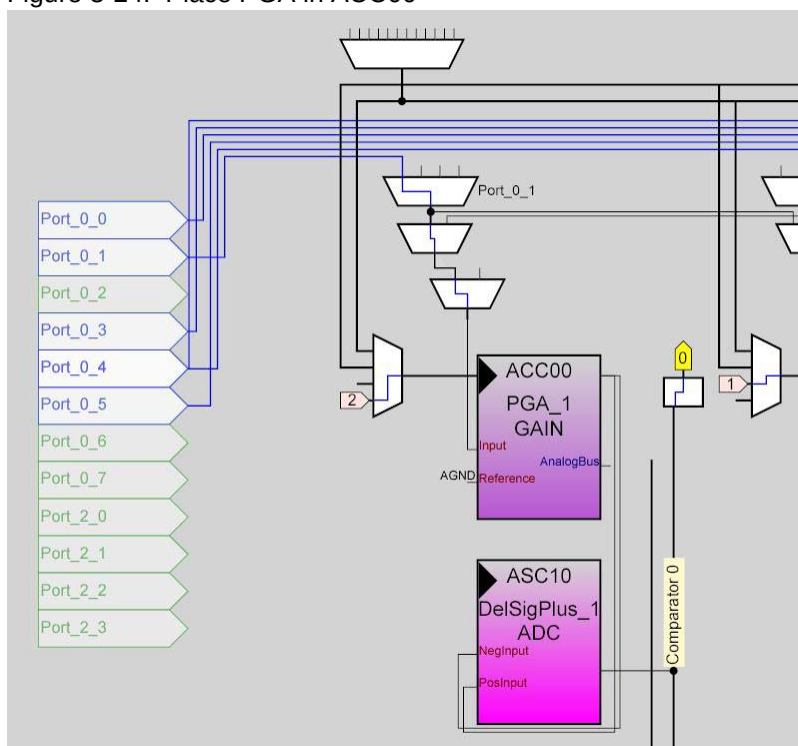
Figure 3-24. Place PGA in ACC00
