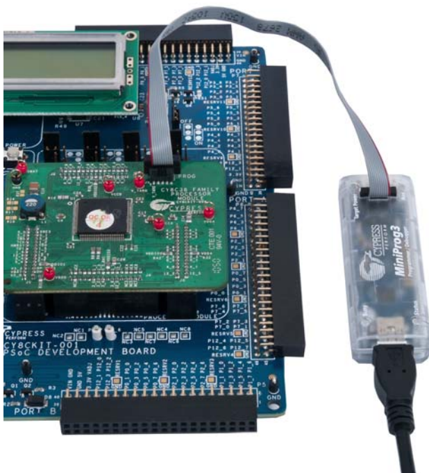
Figure 2-17. Connect MiniProg3 to J5 on CY8CKIT-001 Family Processor Module
