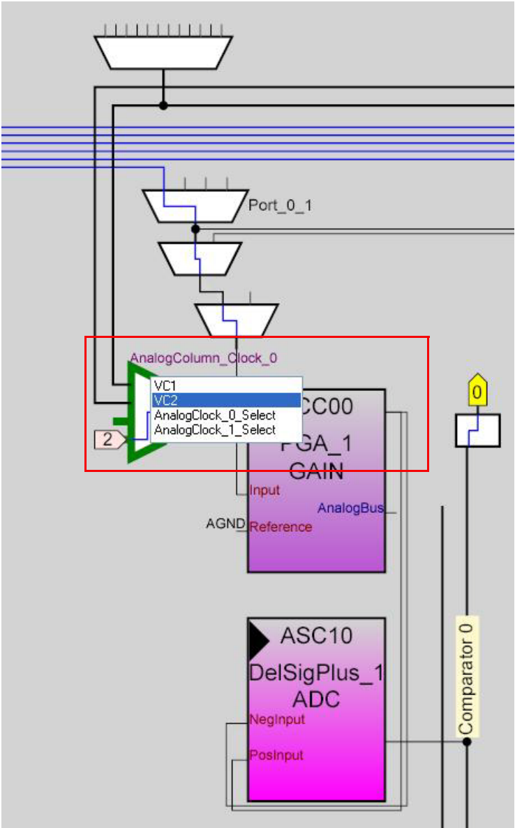
Figure 3-36. AnalogColumn_Clock_0 Connection
