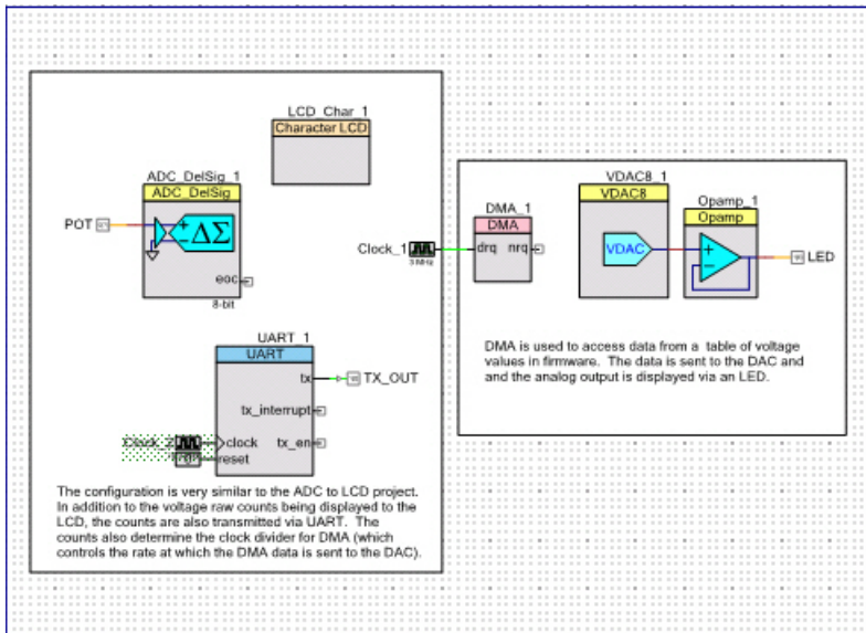
Figure 3-127. Connected Components
