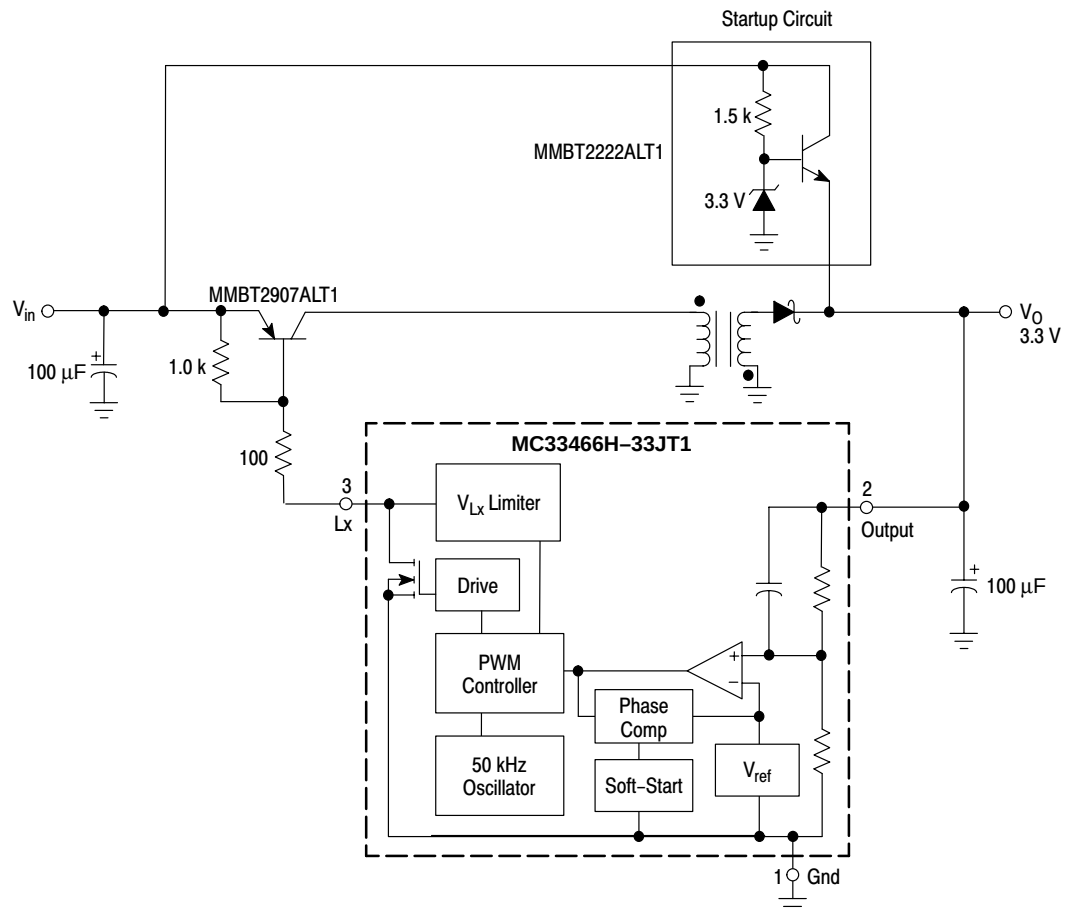
Figure 26. Flyback Application
