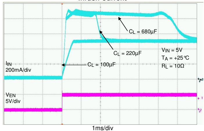
Inrush Current
