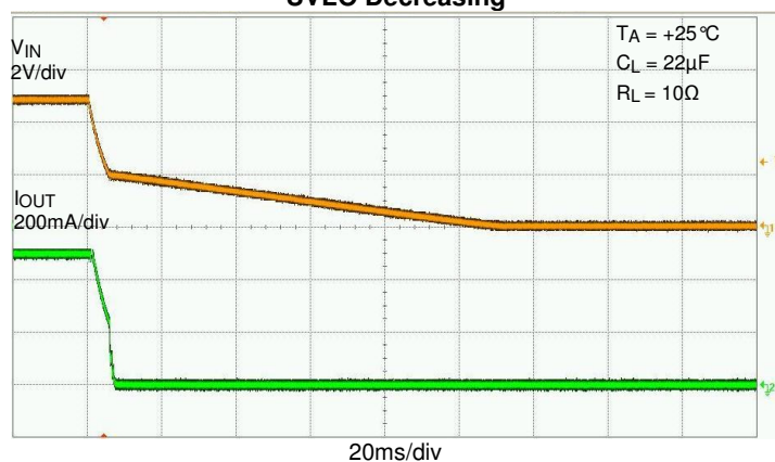
UVLO Decreasing
