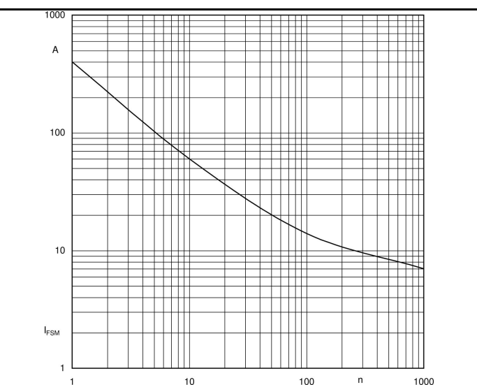
Fig. 4, I_{FSM} current versus number of cycles at 50 Hz
