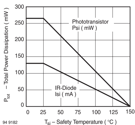
Fig. 1 Derating diagram
