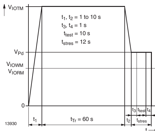
Fig. 2 Test pulse diagram for sample test according to DIN EN 60747-5-2(VDE0884)/ DIN EN 60747-; IEC60747
