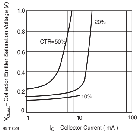
Fig. 12 Collector Emitter Saturation Voltage vs. Collector Current
