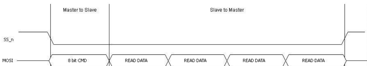
Figure 4-5 3-wire read operation
