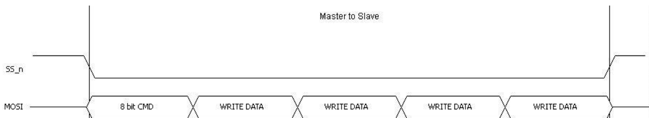
Figure 4-4 3-wire write operation
