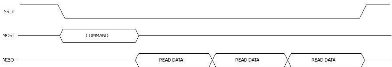
Figure 4-3 4-wire read operation
