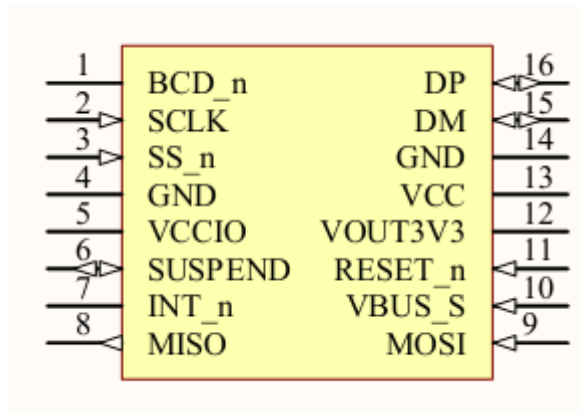
Figure 3-1 TSSOP-16 package schematic symbol
