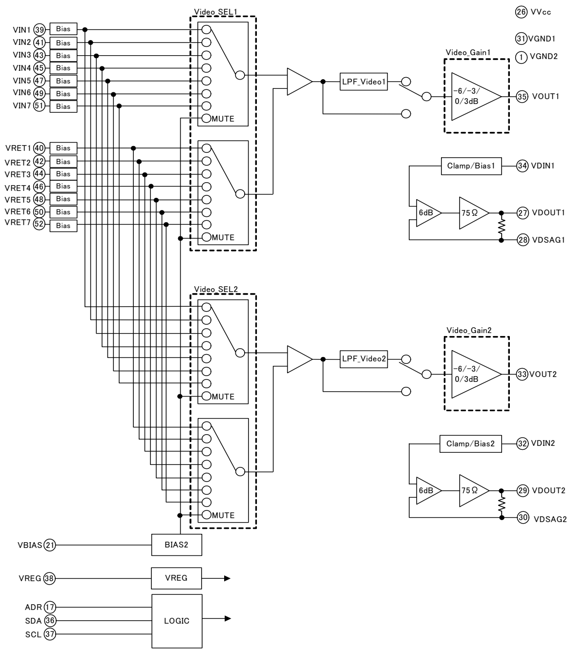
Fig.2 Block Diagram
