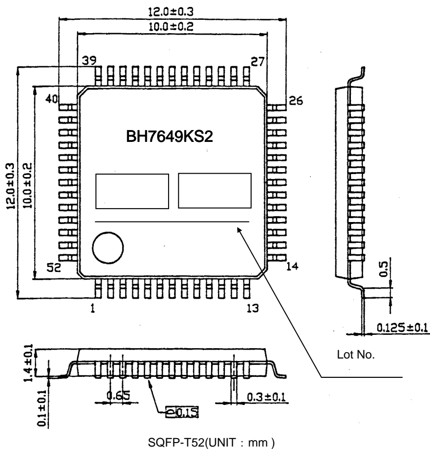
Fig.3 Package outlines
