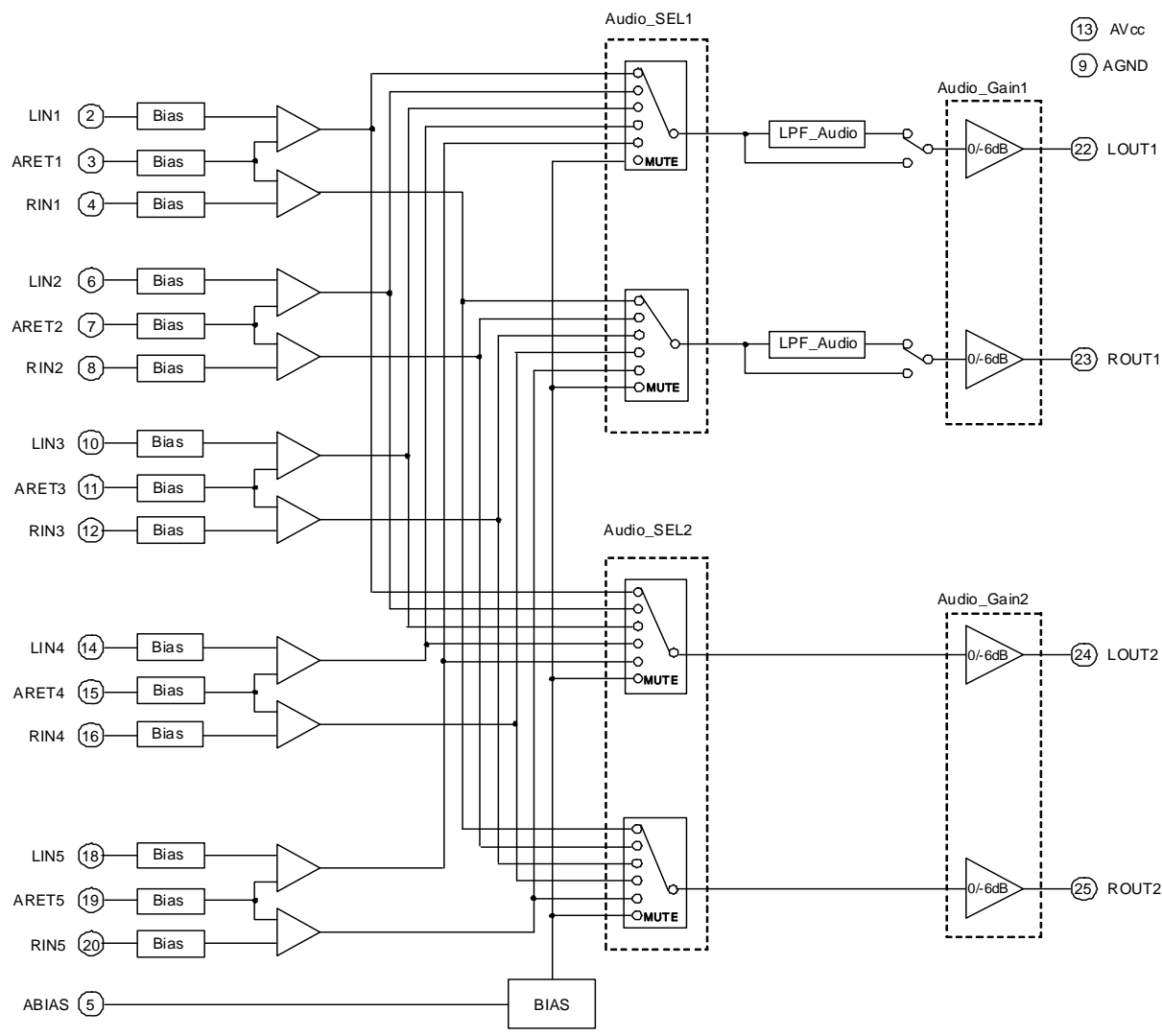
Fig.1 Block Diagram
