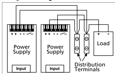
Fig. 27-12 Using distribution terminals
