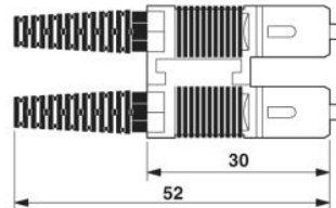
SC duplex connector IP20
