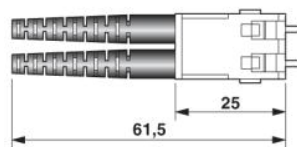
SCRJ plug connector IP20
