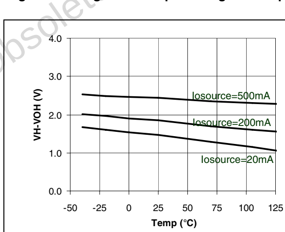
Figure 12. High level output voltage vs temp.
