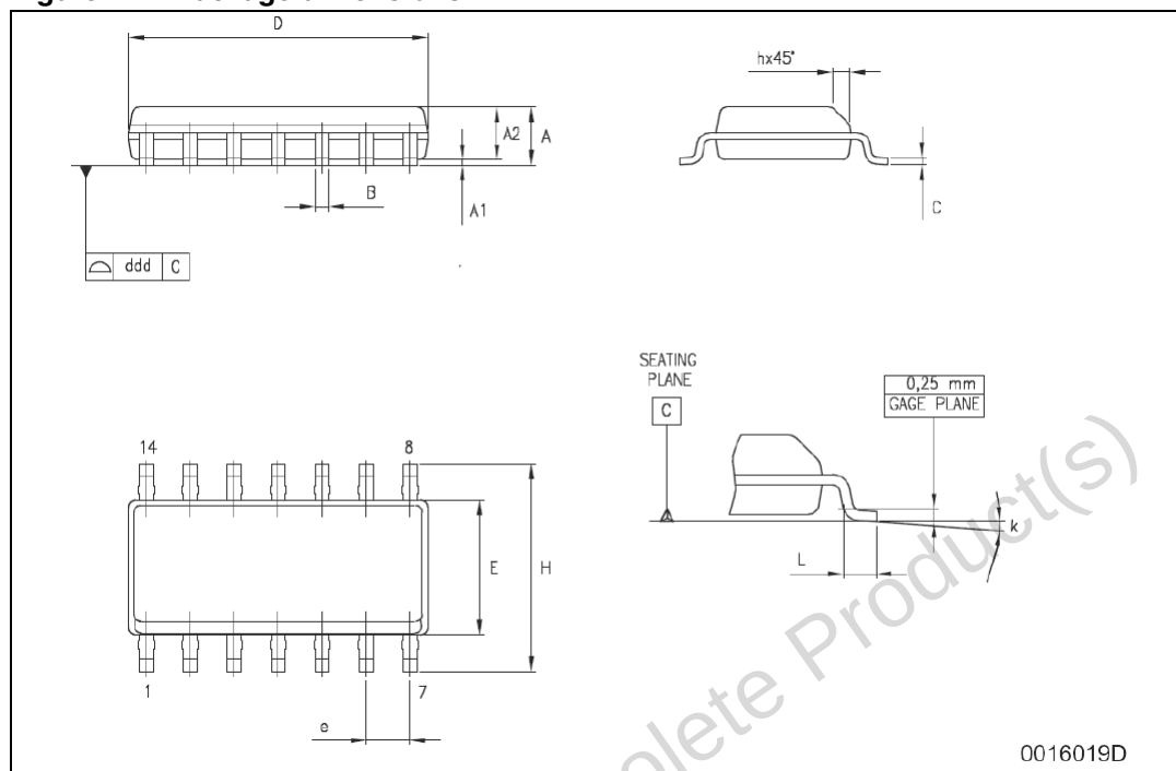
Figure 17. Package dimensions
