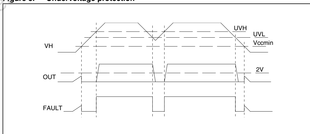
Figure 3. Undervoltage protection
