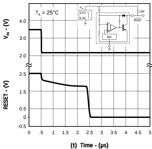
FIGURE 13. — PROPAGATION DELAY — HIGH to LOW
