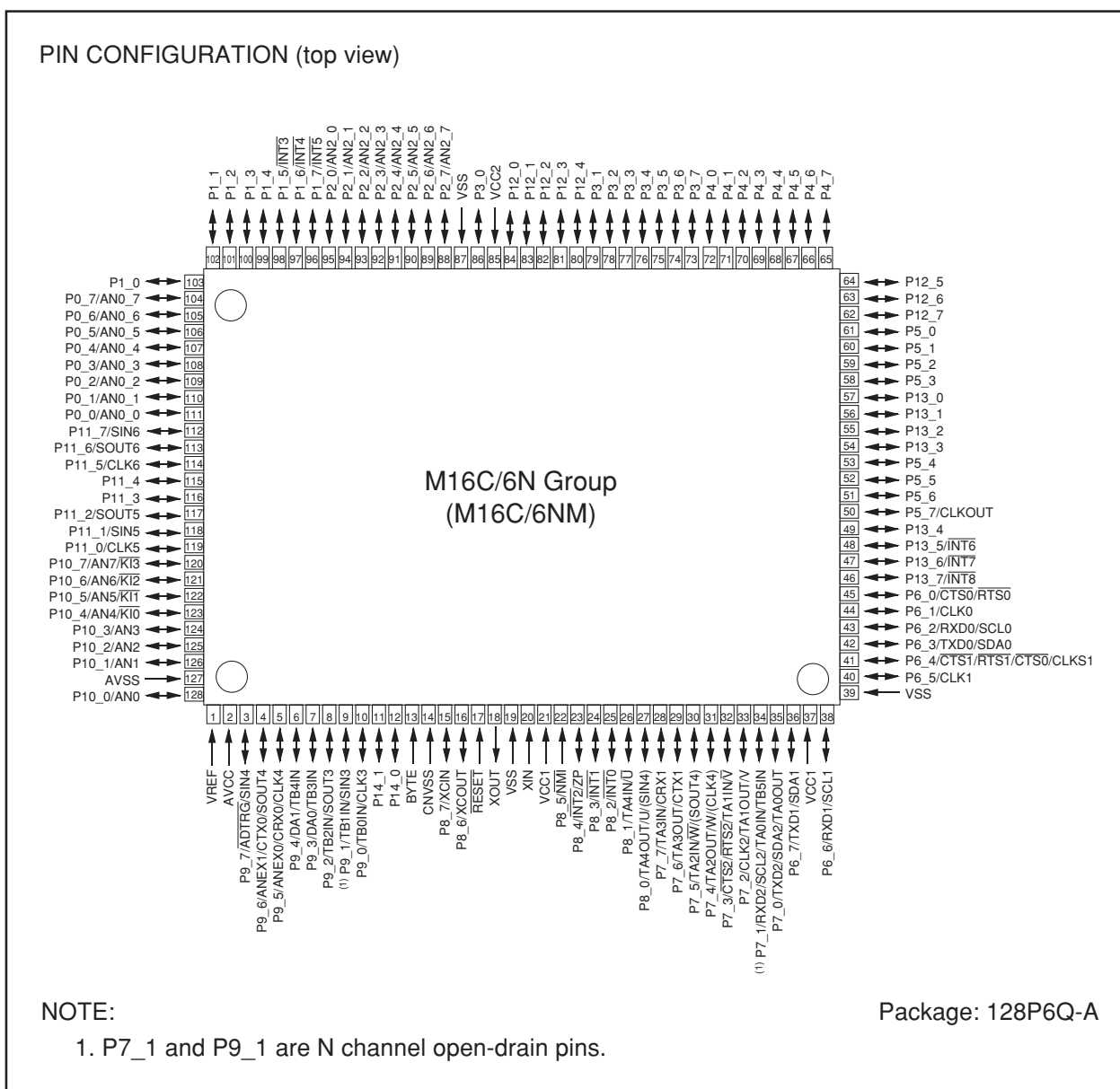
Figure 1.4 Pin Configuration (Top View)
