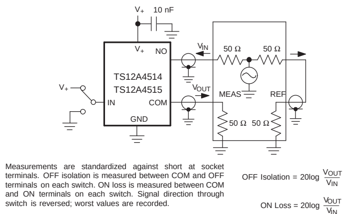
Figure 3. OFF Isolation and ON Loss
