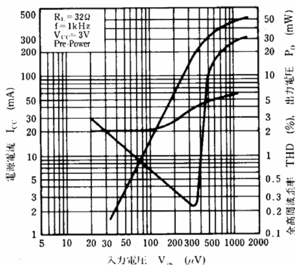
I_{CC}, P_O, \text{THD} - V_{in}
