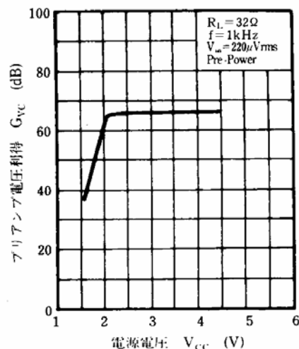
G_{VC} - V_{CC}
