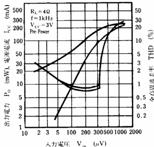
I_{CC}, P_O, \text{THD} - V_{in}
