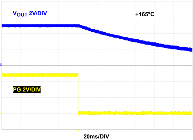
FIGURE 40. OVER-TEMPERATURE PROTECTION
