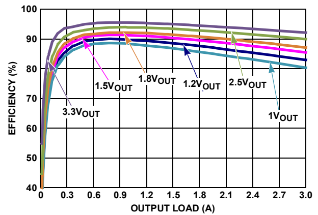
FIGURE 4. EFFICIENCY vs LOAD, 5\text{V}_{IN} CCM
