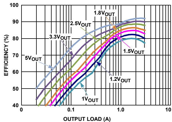
FIGURE 7. EFFICIENCY vs LOAD, 18\text{V}_{IN} DCM
