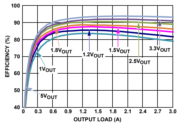
FIGURE 6. EFFICIENCY vs LOAD, 12\text{V}_{IN} CCM
