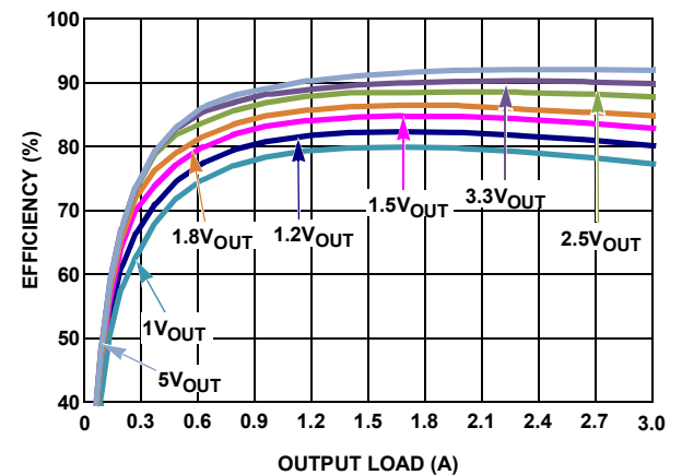
FIGURE 8. EFFICIENCY vs LOAD, 18\text{V}_{IN} CCM
